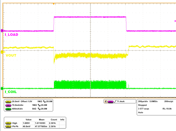
Figure 21. Load transient, V_{IN} 3.6 V, V_{OUT} 1.8 V, I_{OUT} 0 to 100 mA
