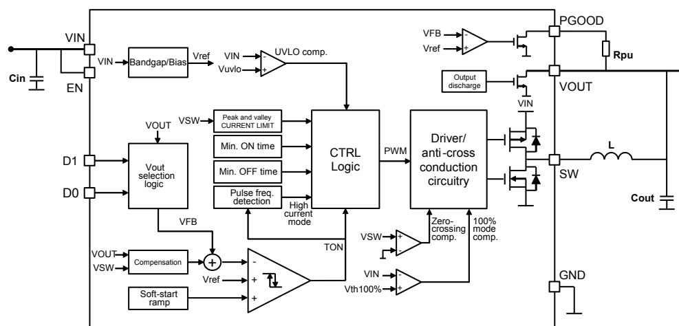
Figure 3. Block diagram
