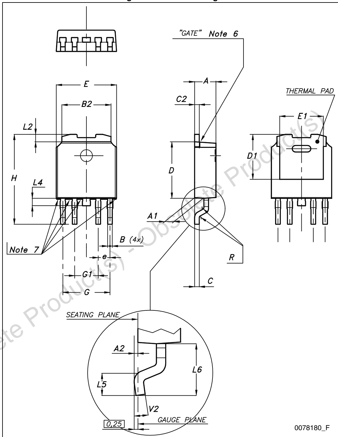
Figure 24. PPAK drawings
