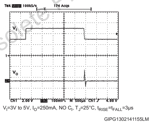
Figure 23. Line transient
