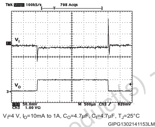
Figure 22. Load transient
