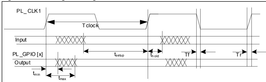
Figure 14. EXPI signal timing waveforms
