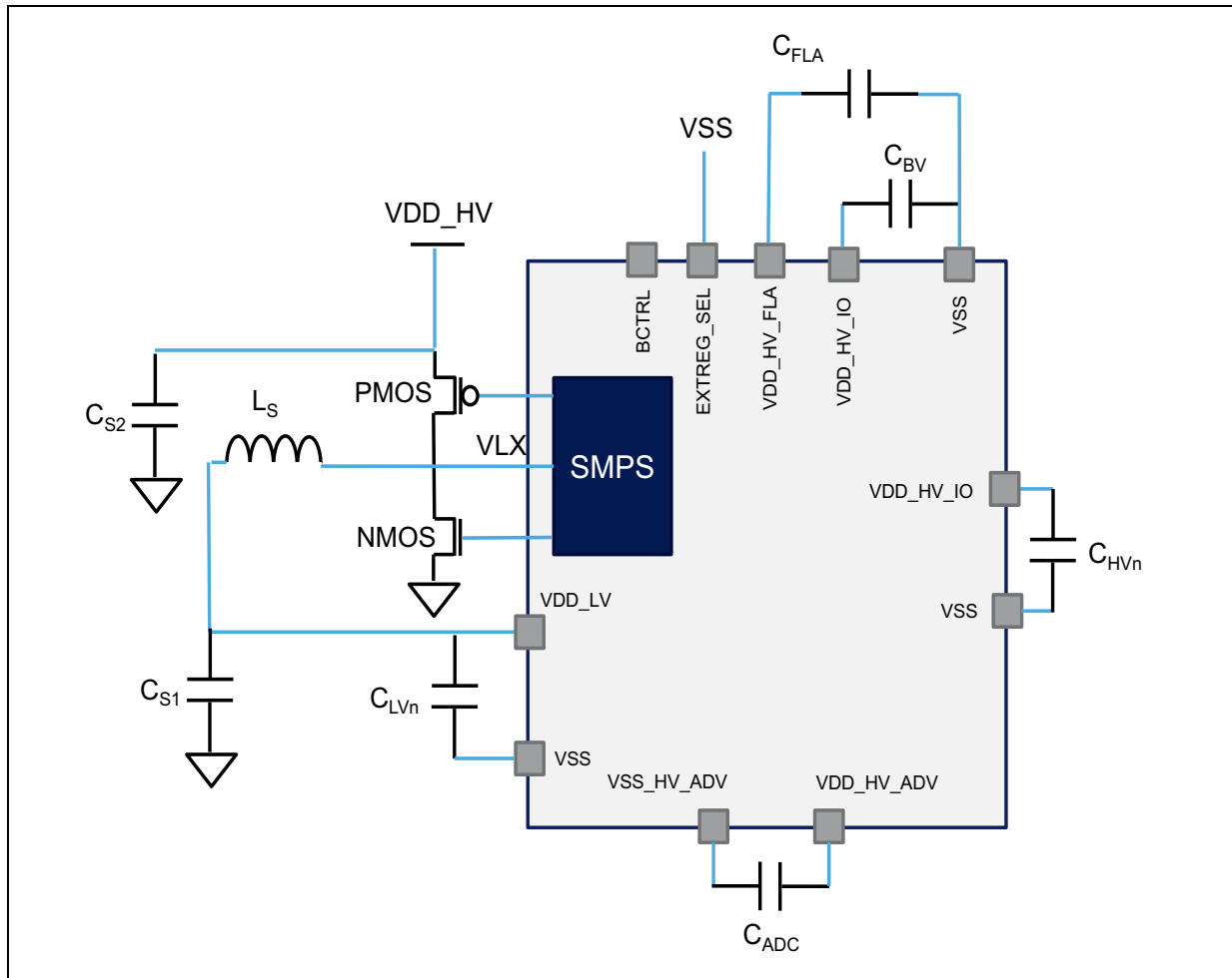
Figure 15. SMPS Regulator Mode
