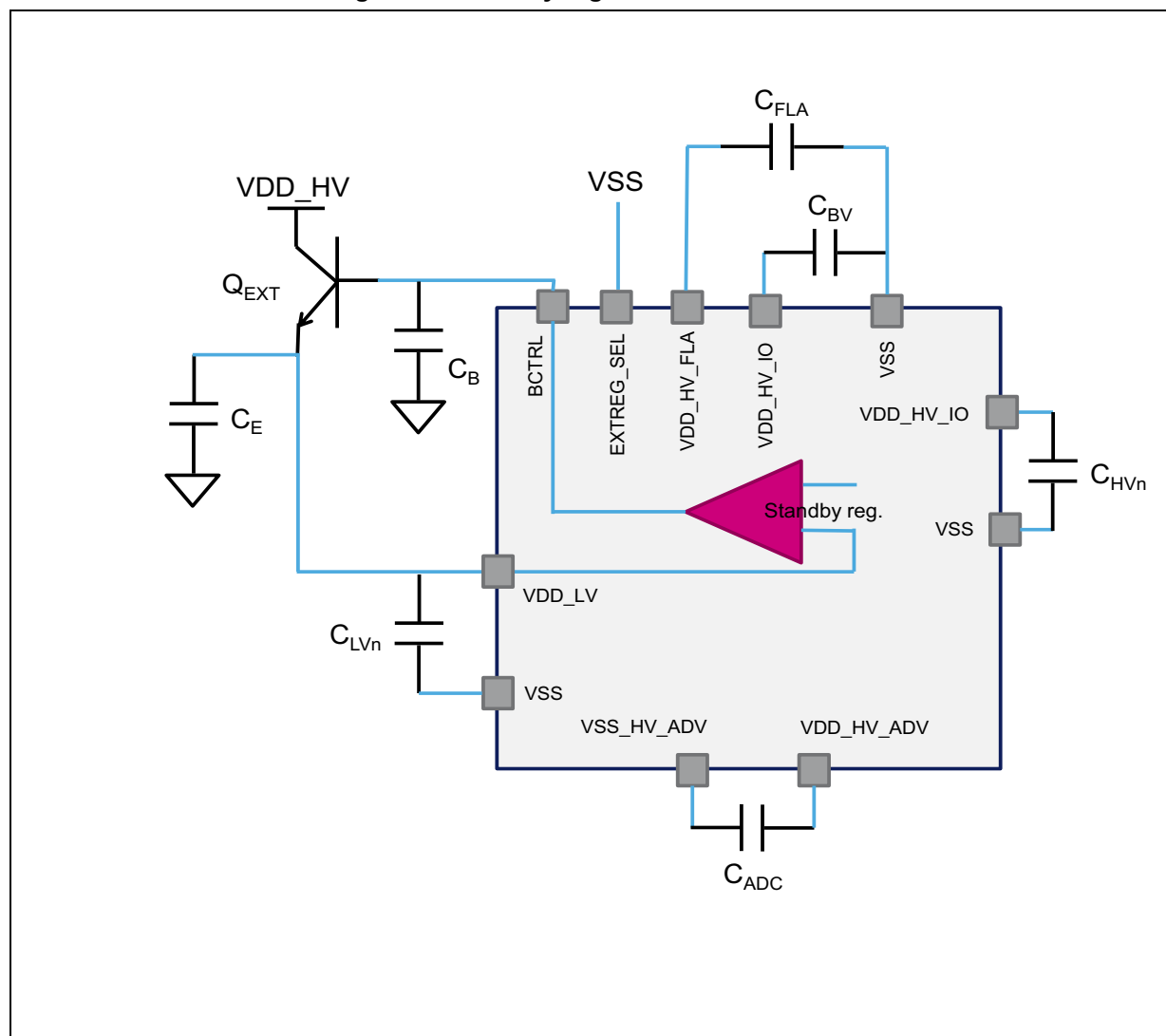
Figure 16. Standby regulator with external ballast mode
