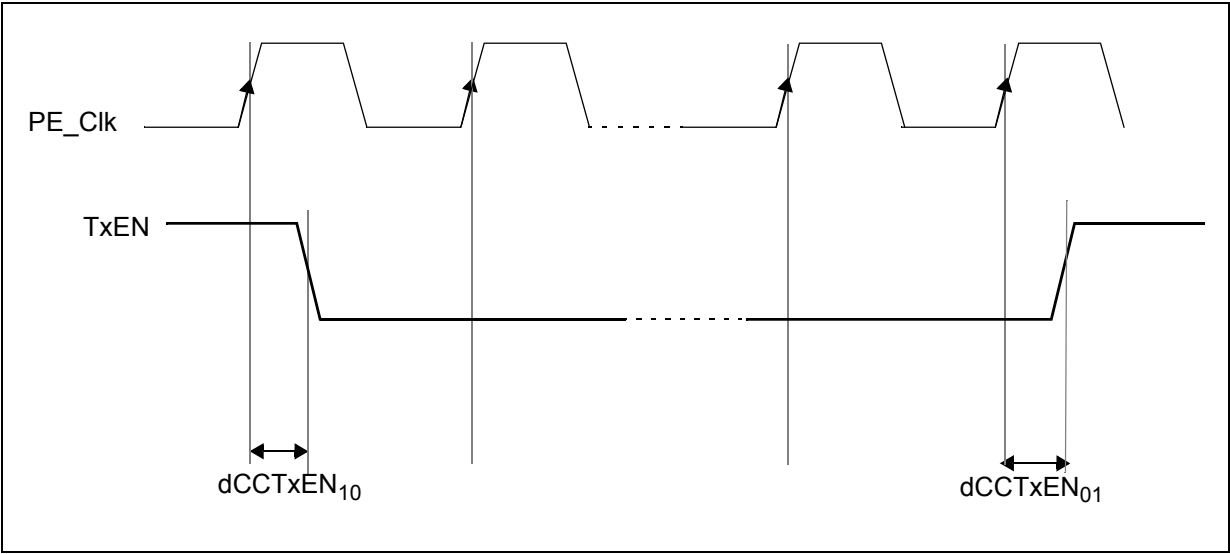
Figure 47. TxEN signal propagation delays
