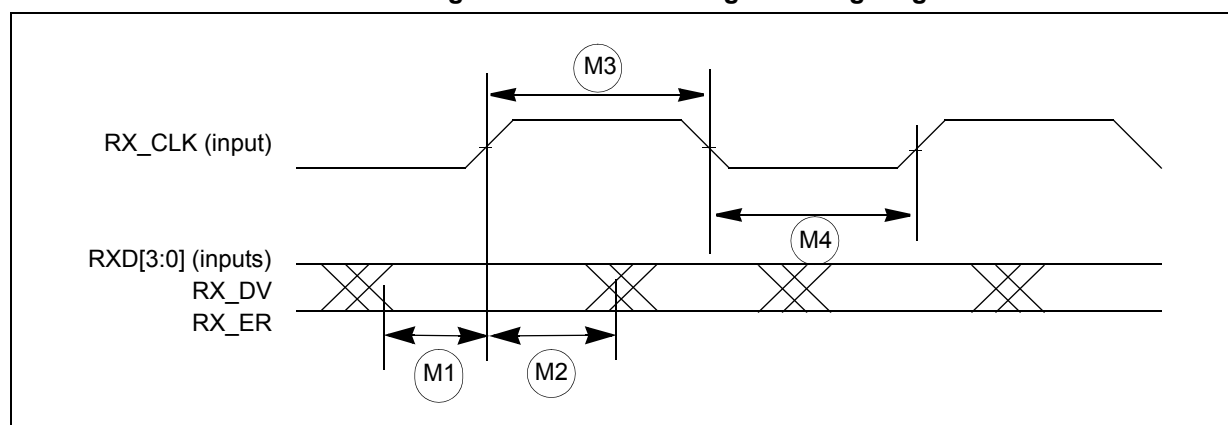
Figure 39. MII receive signal timing diagram
