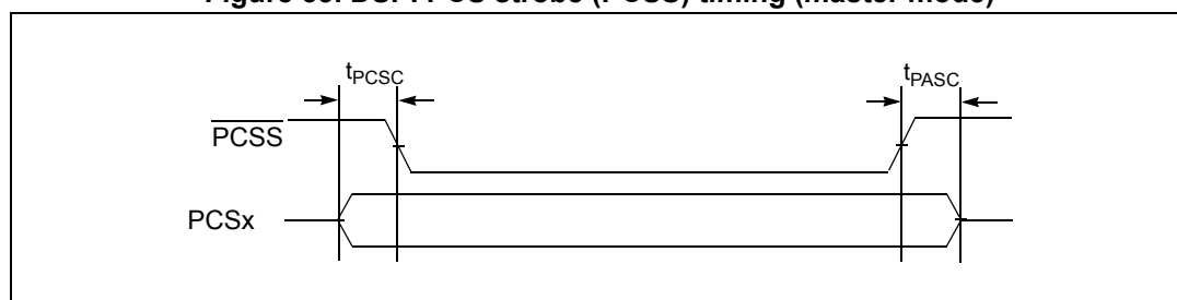
Figure 33. DSPI PCS strobe ( \overline{\text{PCSS}} ) timing (master mode)
