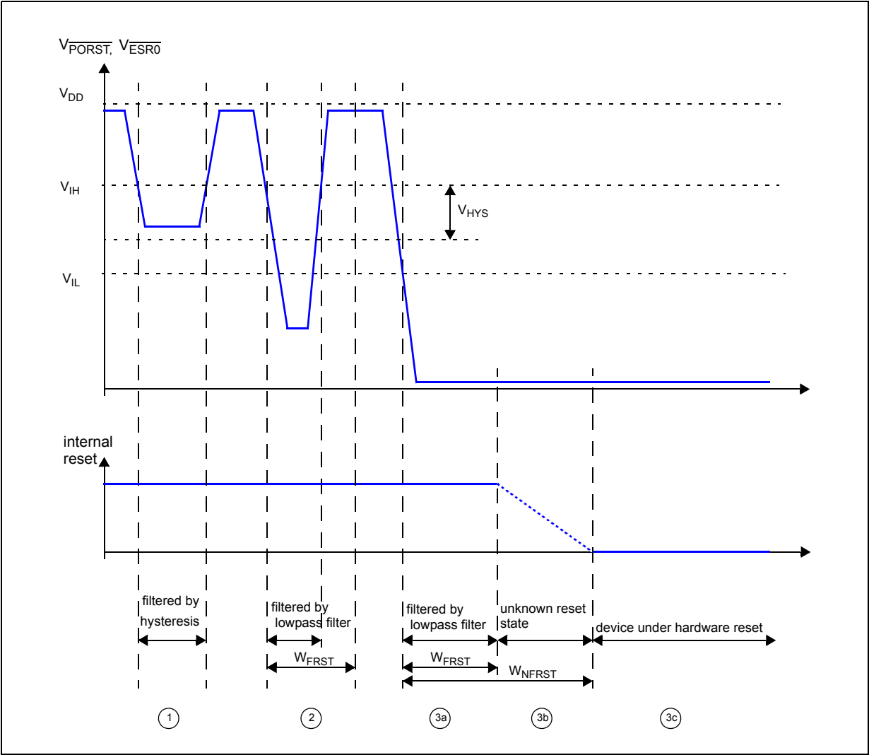
Figure 6. Noise filtering on reset signal
