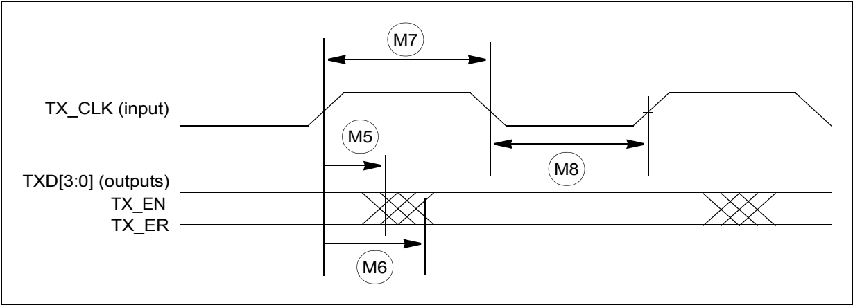
Figure 40. MII transmit signal timing diagram
