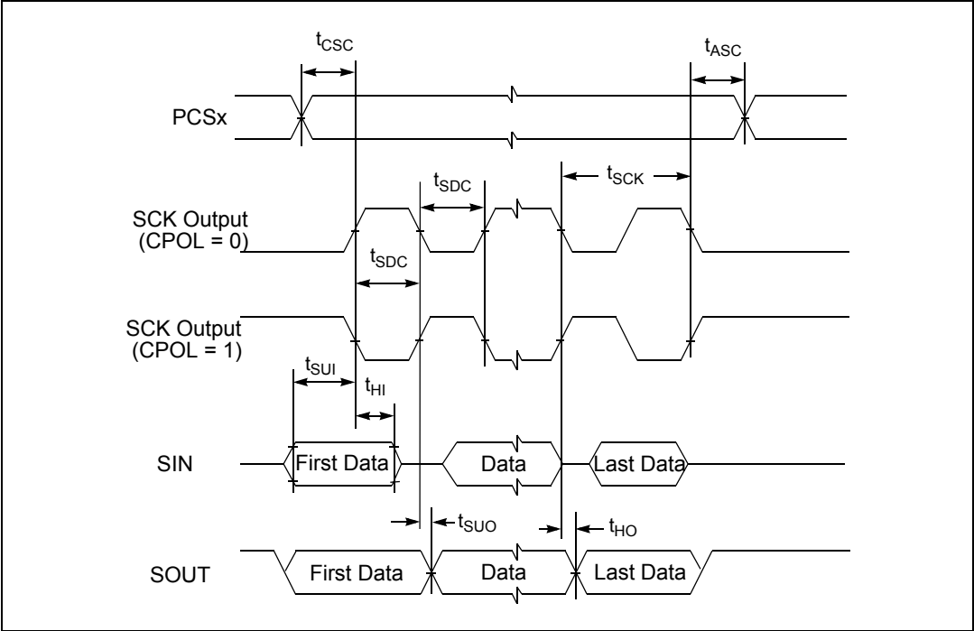
Figure 28. DSPI CMOS master mode — classic timing, CPHA = 0
