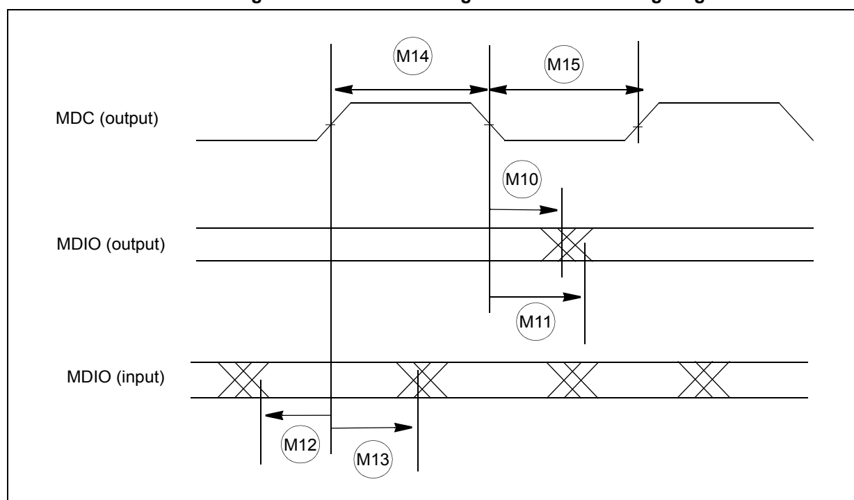
Figure 43. MII serial management channel timing diagram
