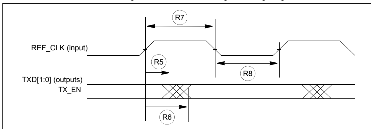
Figure 45. RMII transmit signal timing diagram
