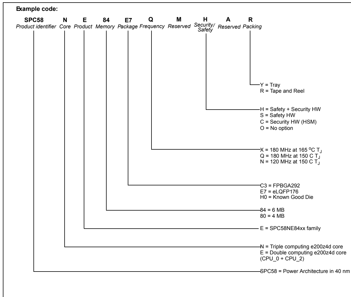
Figure 53. Commercial product scheme
