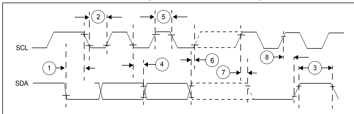
Figure 50. I 2 C input/output timing
