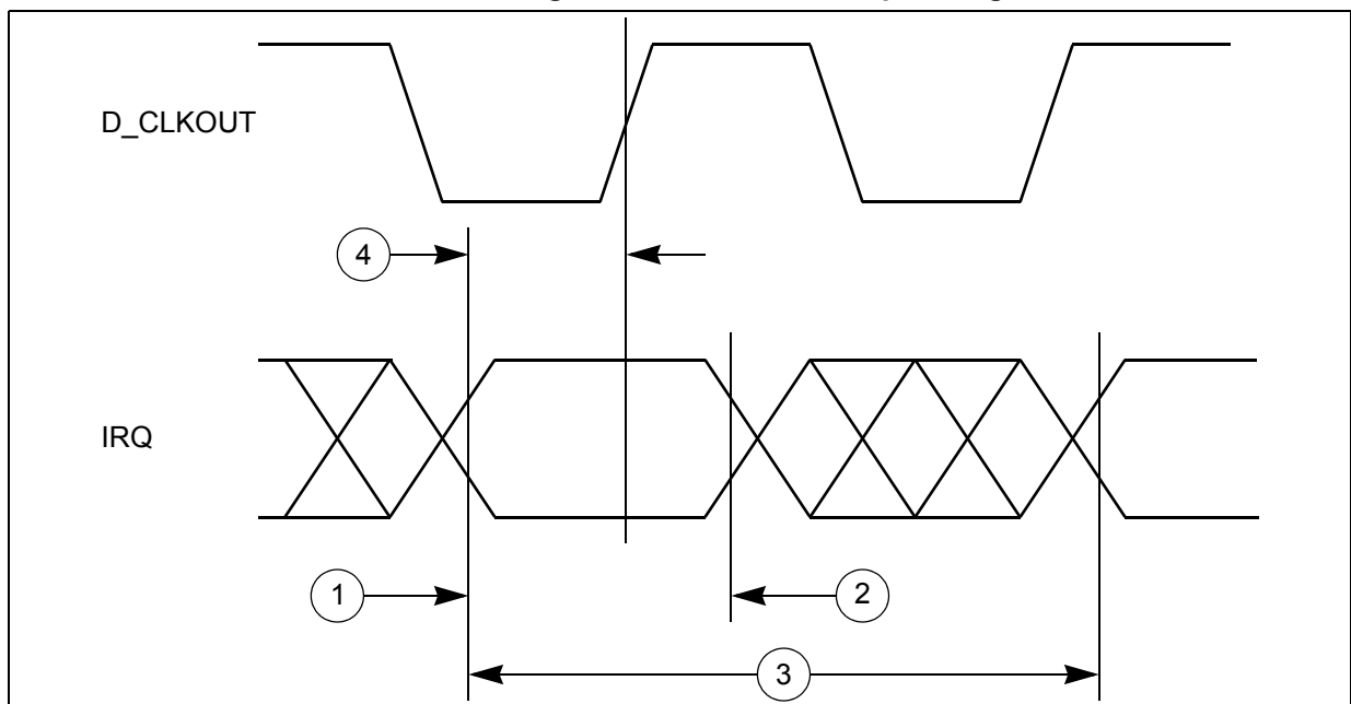
Figure 27. External interrupt timing
