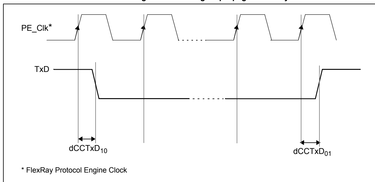
Figure 49. TxD Signal propagation delays
