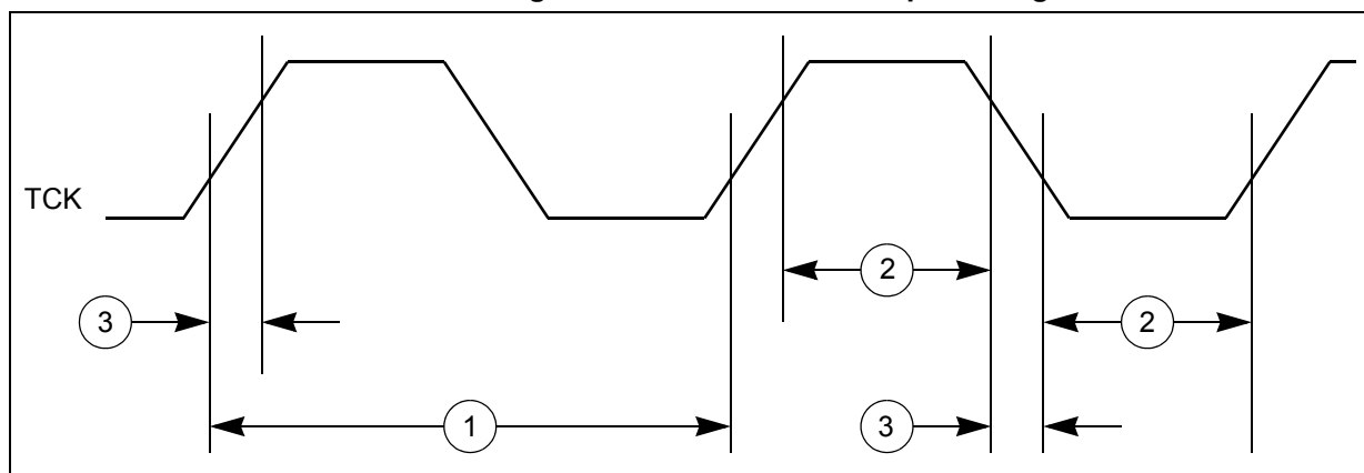
Figure 19. JTAG test access port timing
