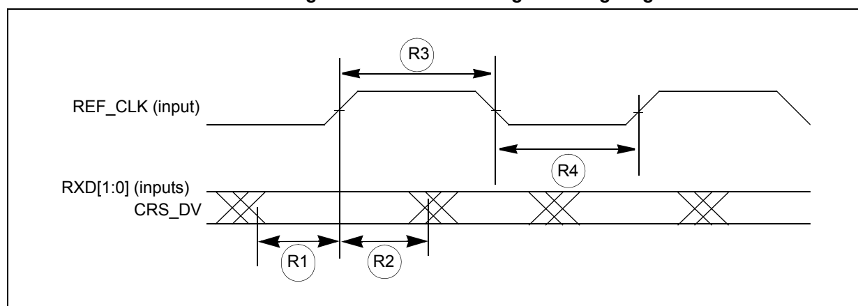
Figure 44. RMII receive signal timing diagram
