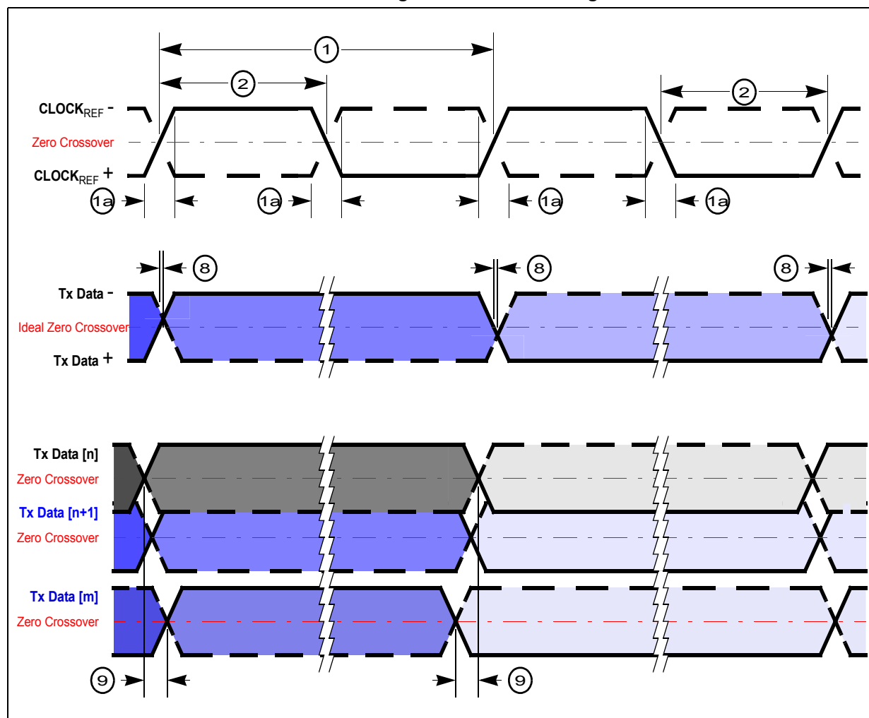
Figure 25. Aurora timings
