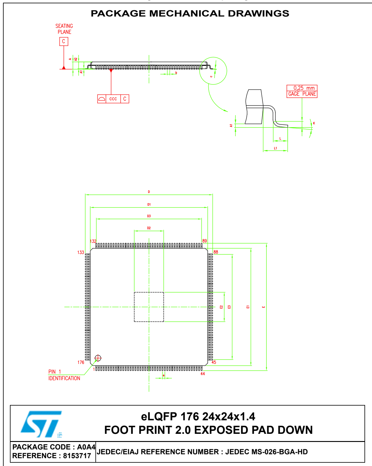
Figure 51. eLQFP176 package outline
