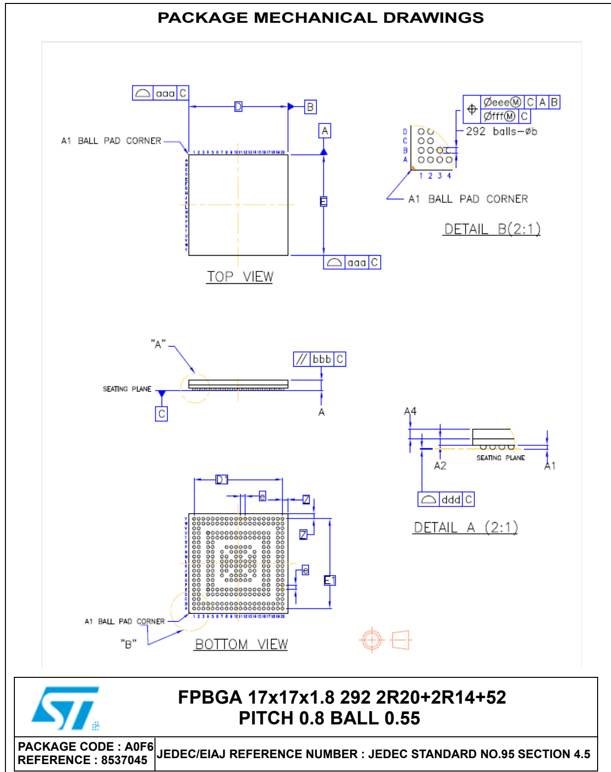
Figure 52. FPBGA292 package outline
