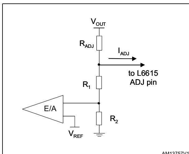
Figure 16. ADJ network
