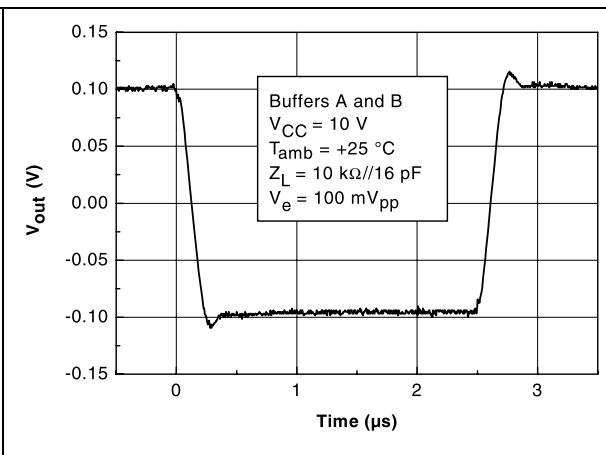
Figure 33. Small signal response - buffers A and B
