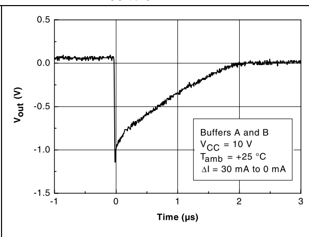
Figure 37. Output voltage response to current transient - buffers A and B, \Delta I = 30 to 0 mA
