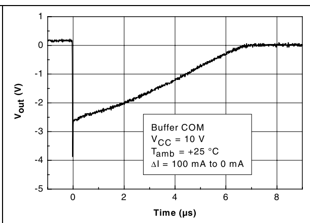
Figure 41. Output voltage response to current transient - buffer COM, \Delta I = 100 to 0 mA
