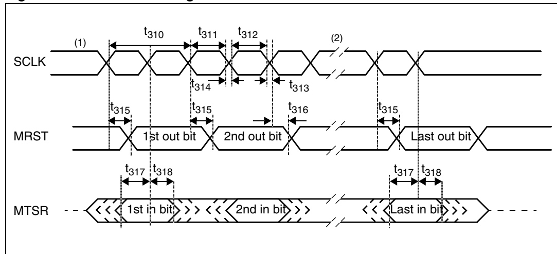
Figure 63. SSC slave timing
