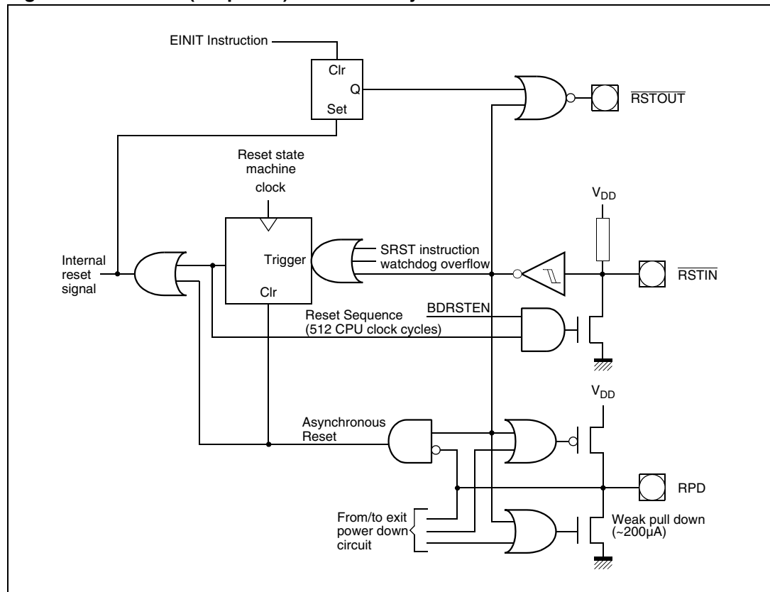
Figure 33. Internal (simplified) reset circuitry
