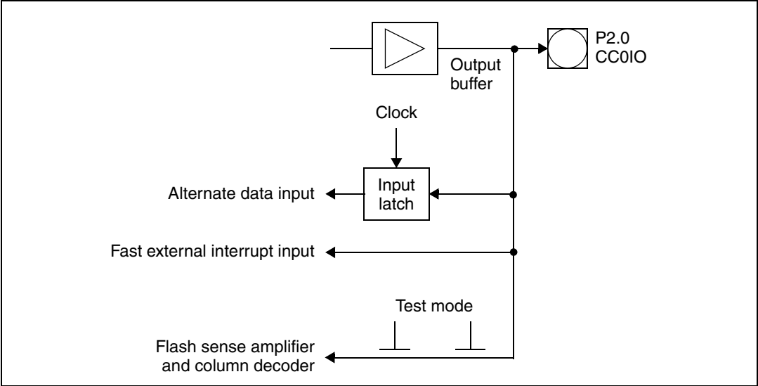
Figure 38. Port2 test mode structure
