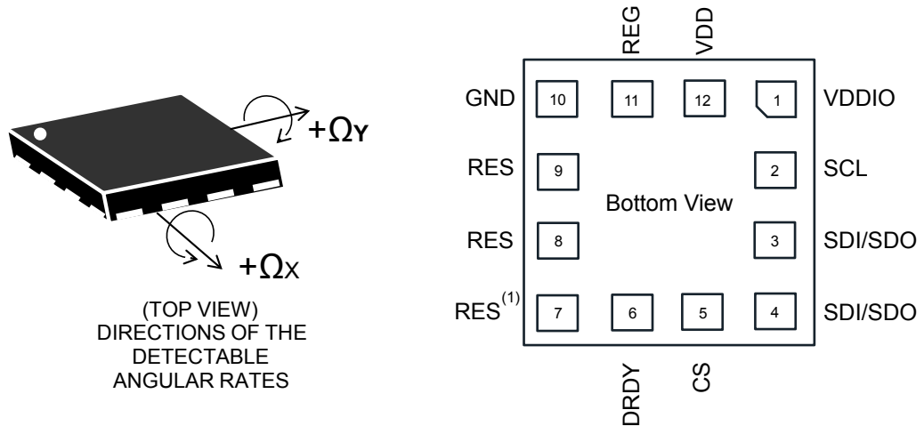
Figure 2. Pin connections
