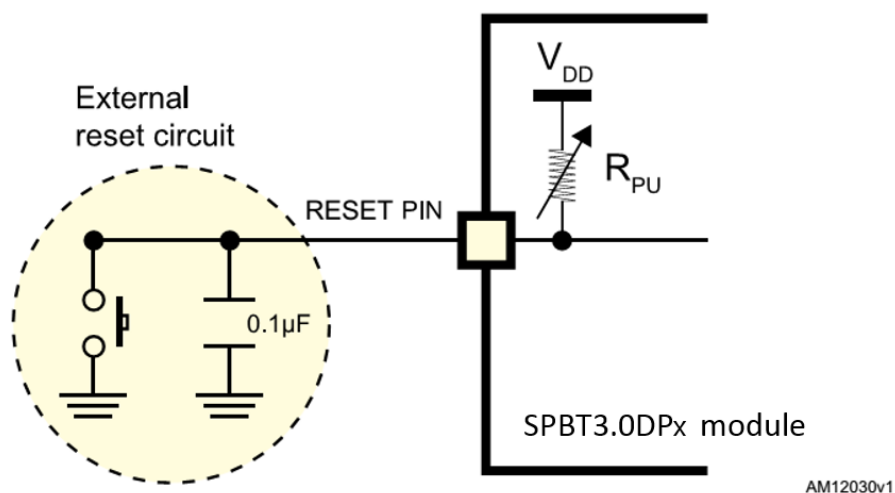
Figure 9. Simple external reset circuit
