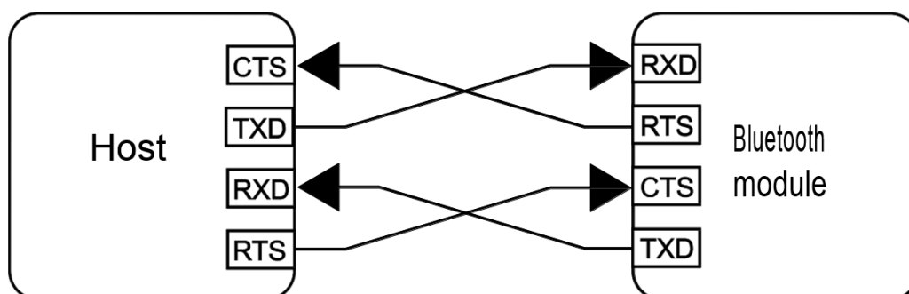
Figure 7. Connection to host device
