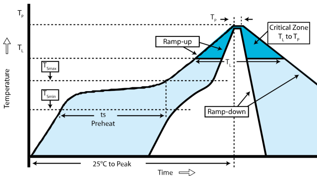
Figure 6. Soldering profile
