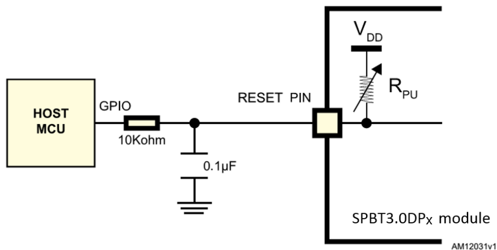
Figure 10. Host controlled reset circuit
