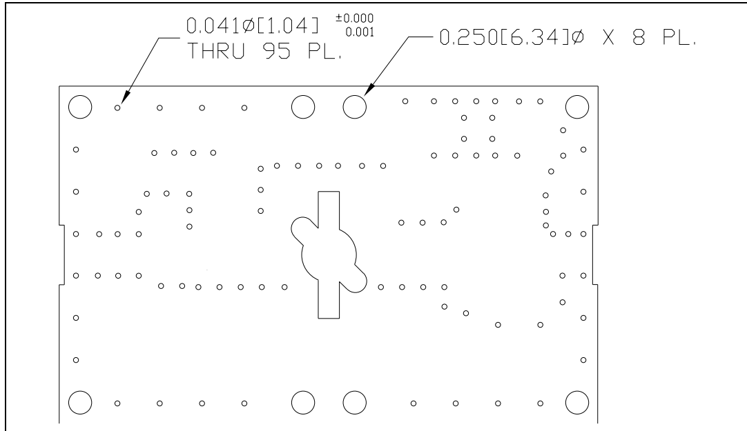
Figure 17. Test fixture component layout
