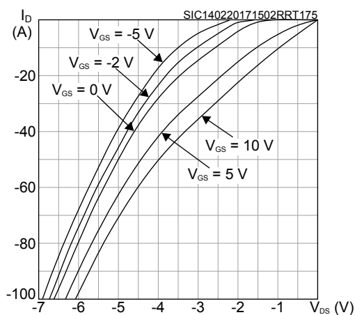
Figure 15. Reverse conduction characteristics ( T_J = 175^\circ\text{C} )
