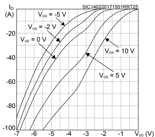
Figure 14. Reverse conduction characteristics ( T_J = 25^\circ\text{C} )
