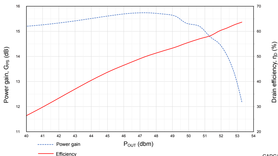
Figure 1. Power Gain and drain efficiency vs output power at 1450 MHz (on Doherty test fixture)
