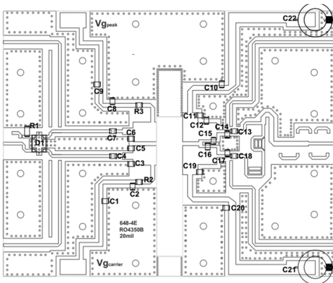
Figure 2. Test circuit layout
