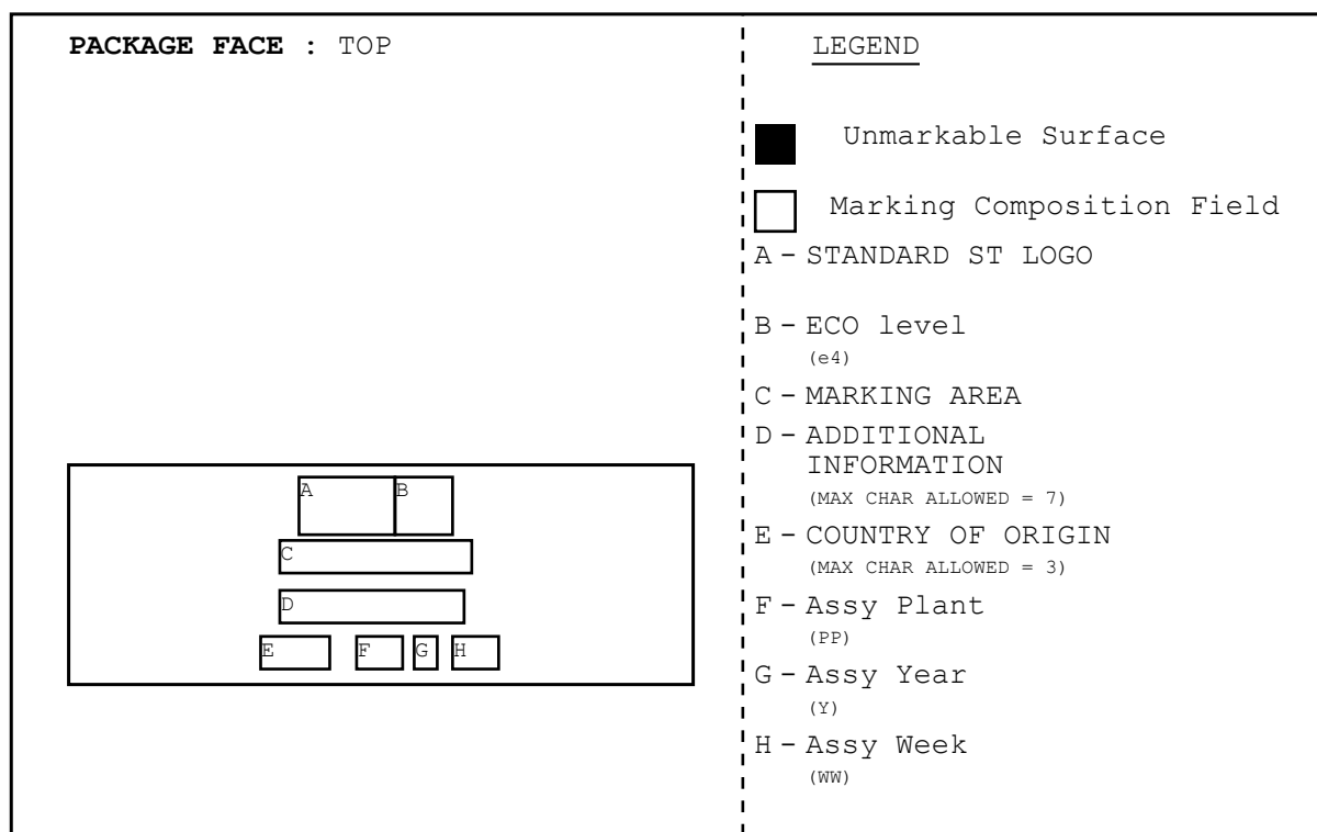
Figure 5. Marking composition
