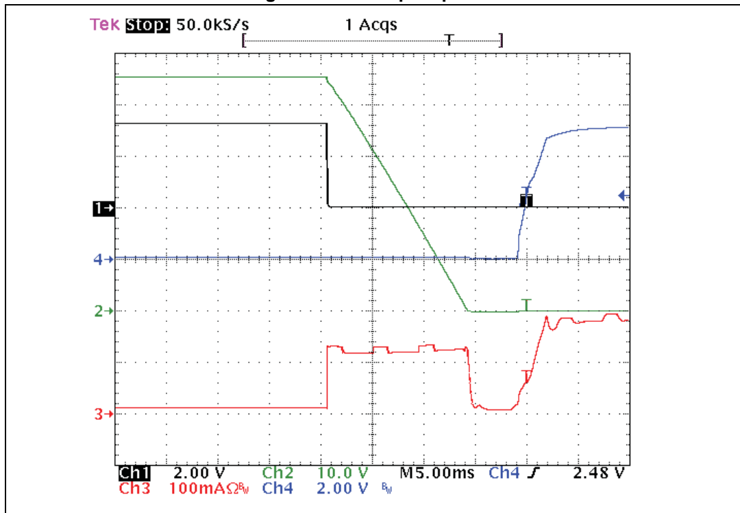
Figure 12. Wakeup sequence
