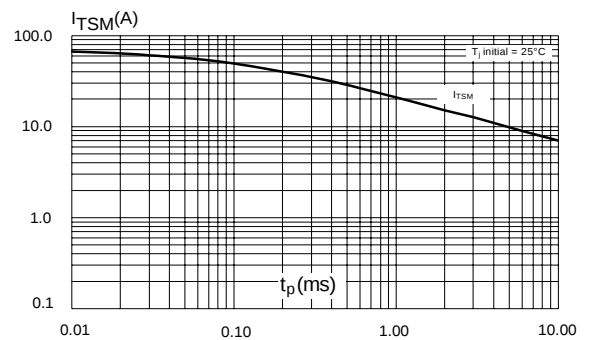
Figure 10: Non-repetitive surge peak on-state current for sinusoidal pulse ( t_p < 10 ms)
