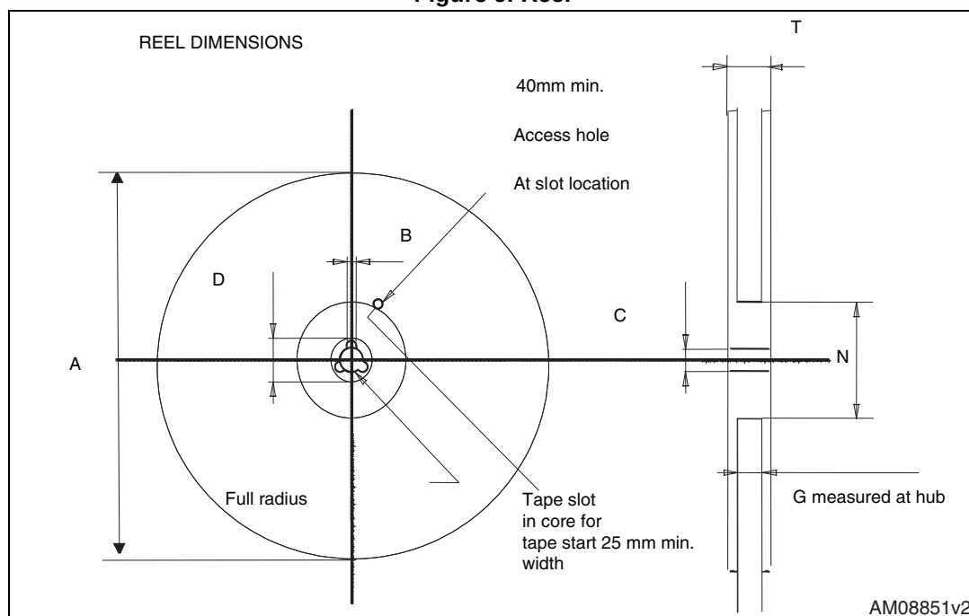
Figure 9. Reel
