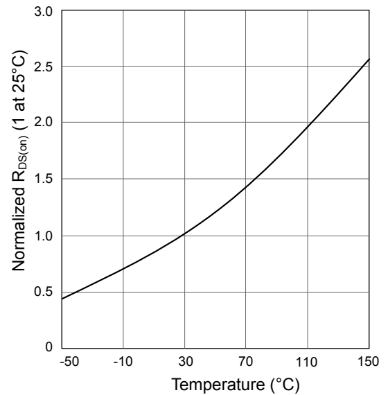
Figure 9. Typ R_{DS(on)_x} vs T_J , normalized at 25^\circ\text{C}
