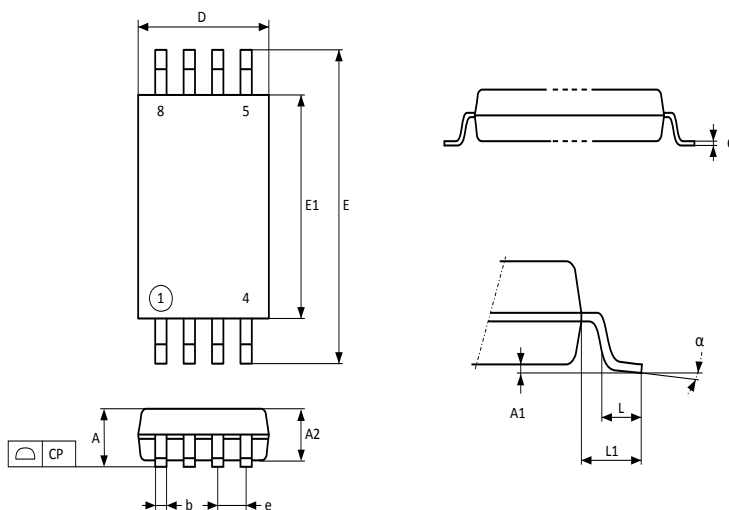
Figure 17. TSSOP8 - Outline
