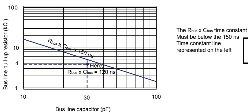
Figure 13. Maximum R_{bus} value vs. bus parasitic capacitance ( C_{bus} ) for an I 2 C bus at f_C = 1 MHz
