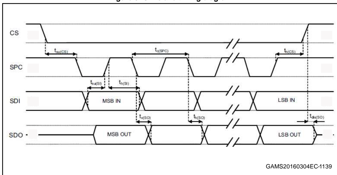
Figure 3: SPI slave timing diagram
