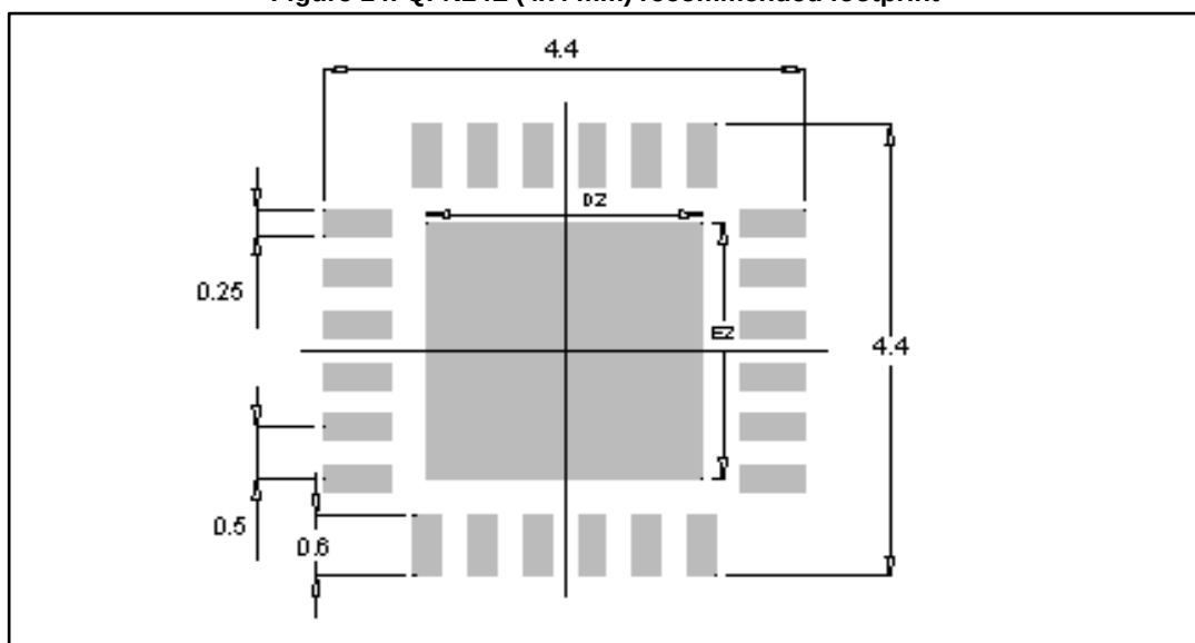
Figure 14: QFN24L (4x4 mm) recommended footprint
