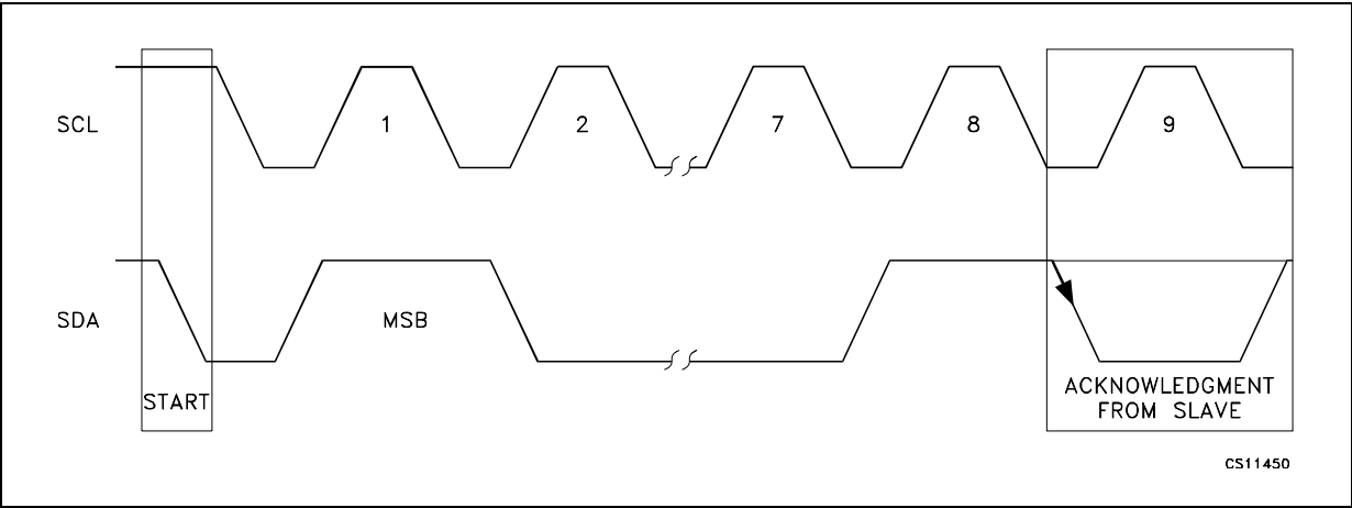
Figure 8. Acknowledge on the I 2 C bus
