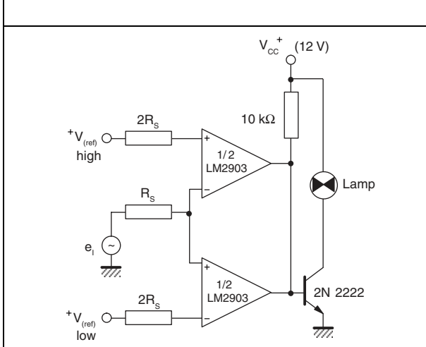
Figure 15. Limit comparator
