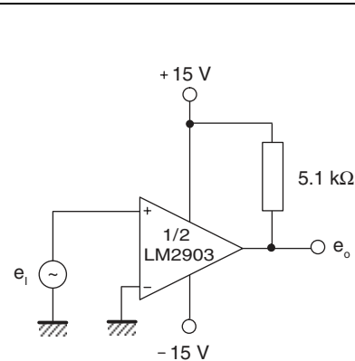
Figure 16. Split-supply applications - zero crossing detector
