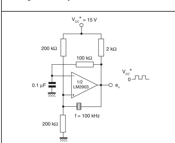
Figure 17. Crystal controlled oscillator
