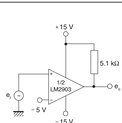
Figure 18. Comparator with a negative reference
