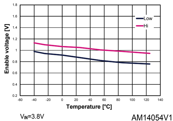
Figure 22. Enable thresholds vs. temperature
