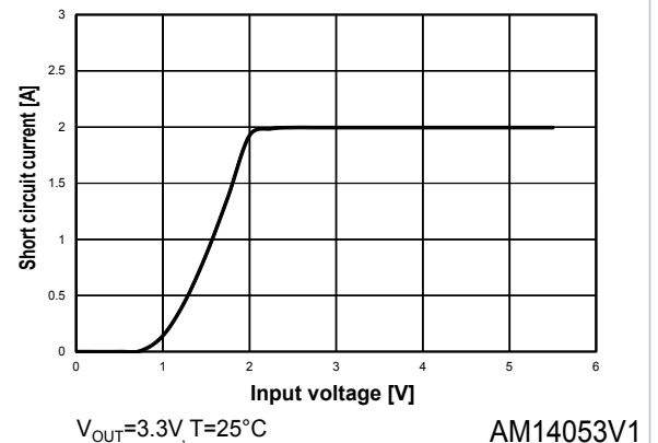
Figure 21. Short-circuit current vs. input voltage
