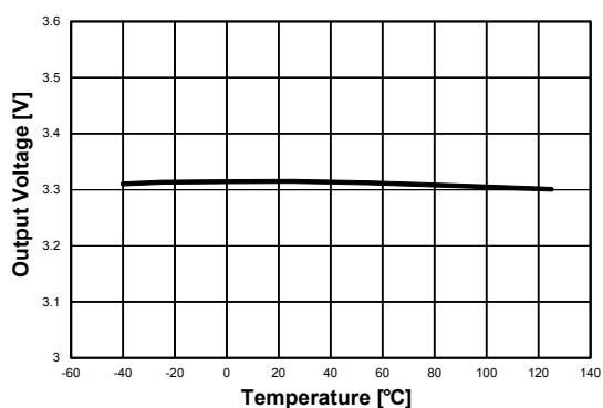
Figure 8. Output voltage vs. temperature ( V_{OUT} = 3.3 V , I_{OUT} = 5 mA )
