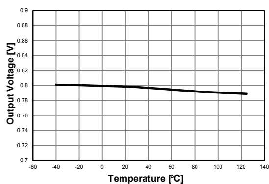
Figure 11. Output voltage vs. temperature ( V_{OUT} = V_{ADJ} , I_{OUT} = 1.2 A )
