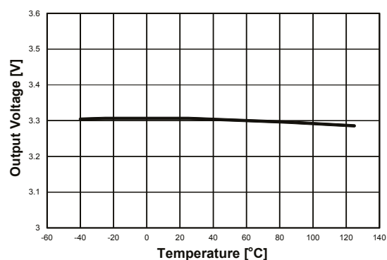
Figure 9. Output voltage vs. temperature ( V_{OUT} = 3.3 V , I_{OUT} = 1.2 A )
