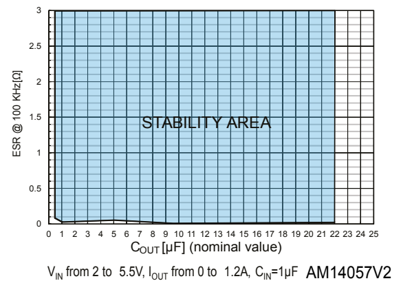
Figure 25. Stability plan vs. C_{OUT} , ESR
