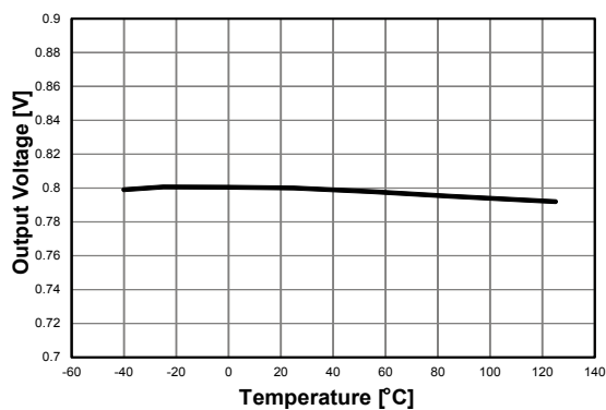
Figure 10. Output voltage vs. temperature ( V_{OUT} = V_{ADJ} , I_{OUT} = 5 mA )
