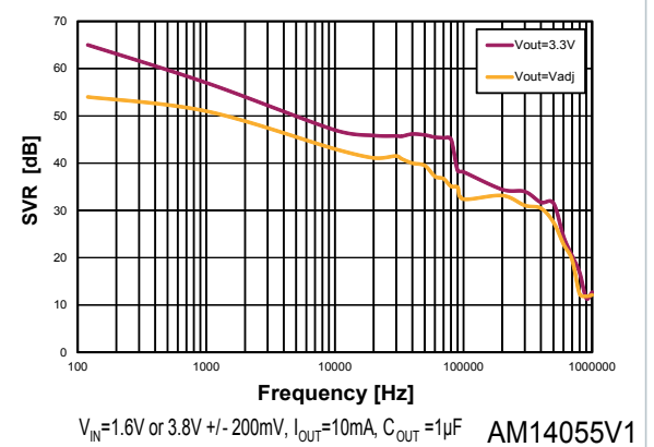
Figure 23. SVR vs. frequency
