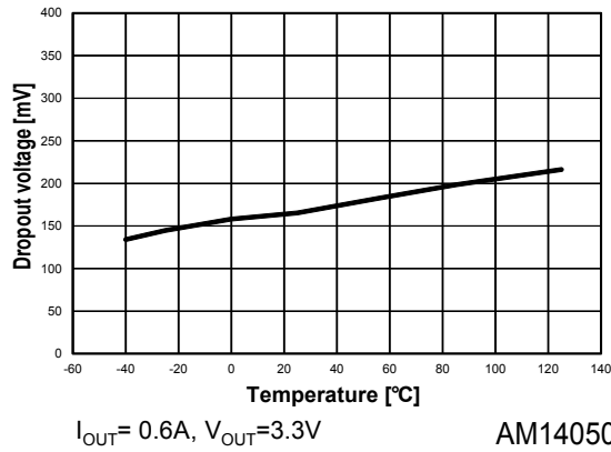
Figure 18. Dropout voltage vs. temperature (I_{OUT} = 600 \text{ mA})
