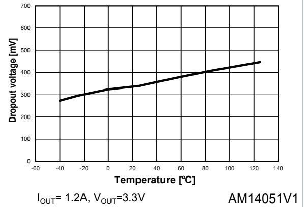
Figure 19. Dropout voltage vs. temperature (I_{OUT} = 1.2 A)
