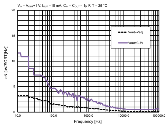
Figure 24. Output noise spectral density
