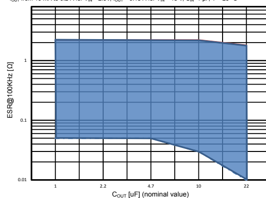
Figure 26. Stability plan ( V_{OUT} = V_{ADJ} )
