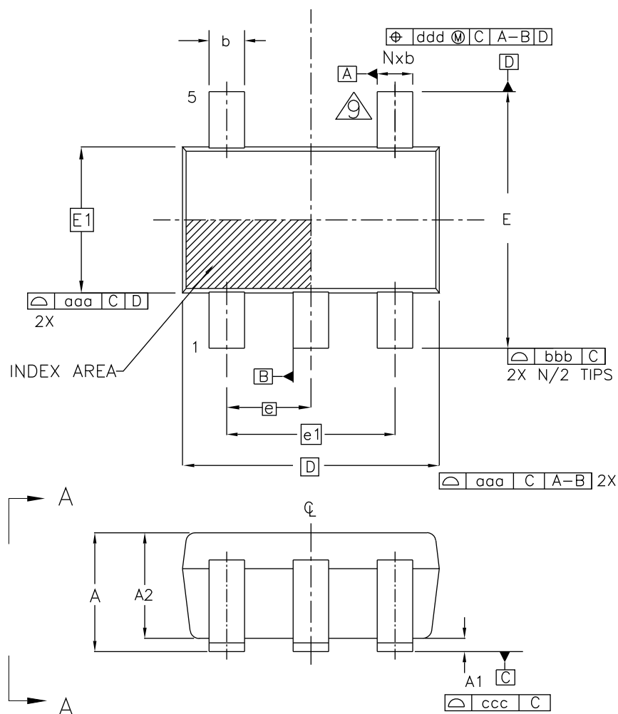
Figure 36. SOT23-5L package outline (option B)
