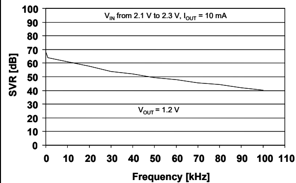
Figure 24. Supply voltage rejection vs. frequency ( V_{OUT} = 1.2\text{ V} )
