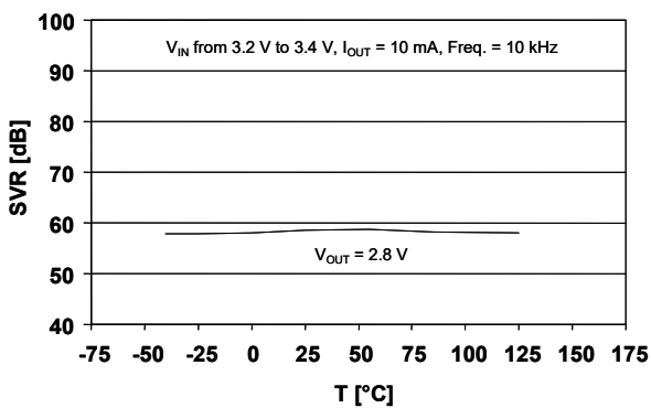
Figure 23. Supply voltage rejection vs. temperature ( V_{OUT} = 2.8\text{ V} )
