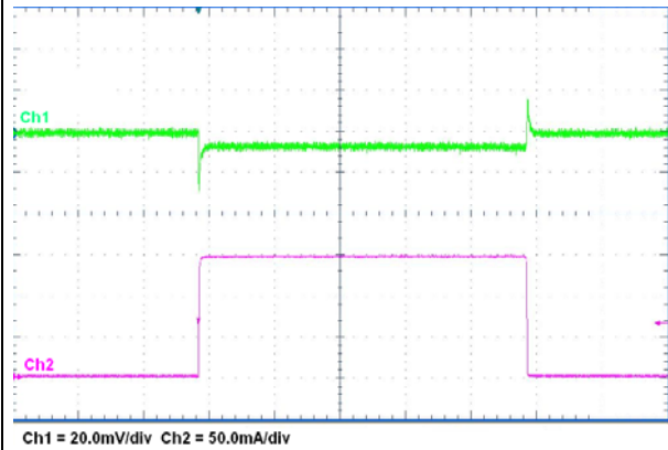
Figure 13. Load transient
