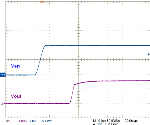
Figure 15. Enable transient
