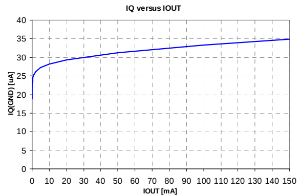
Figure 11. Quiescent current vs. I_{OUT}
