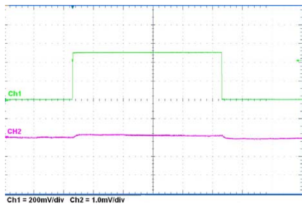
Figure 14. Line transient
