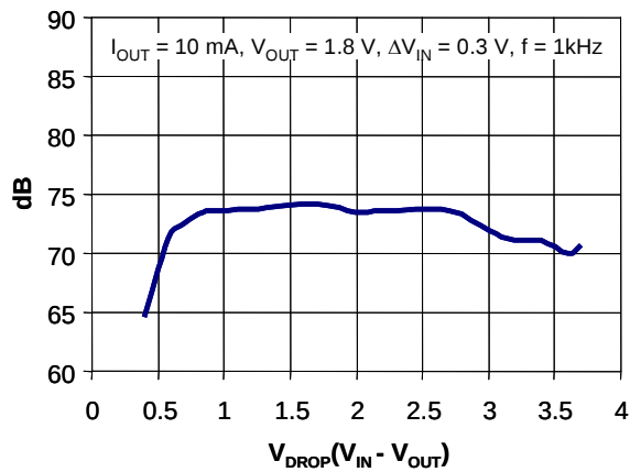
Figure 10. SVR vs. drop
