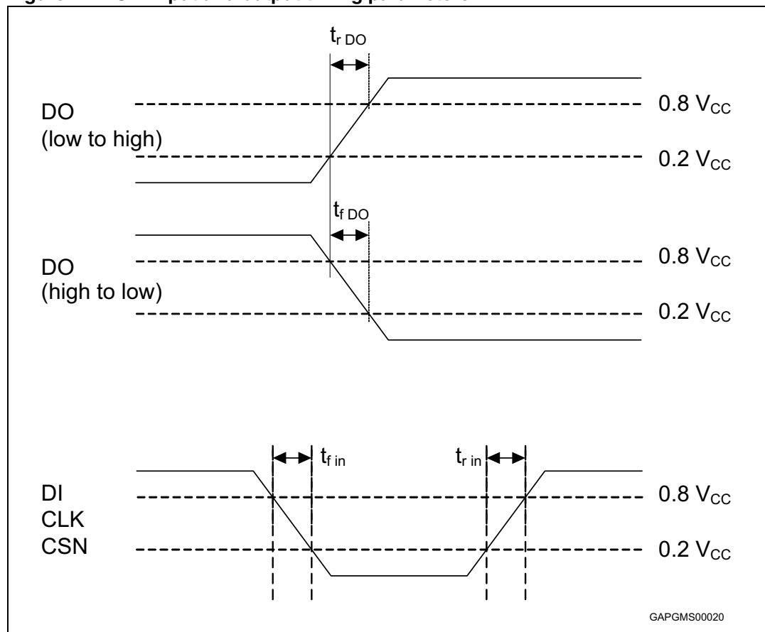
Figure 17. SPI input and output timing parameters
