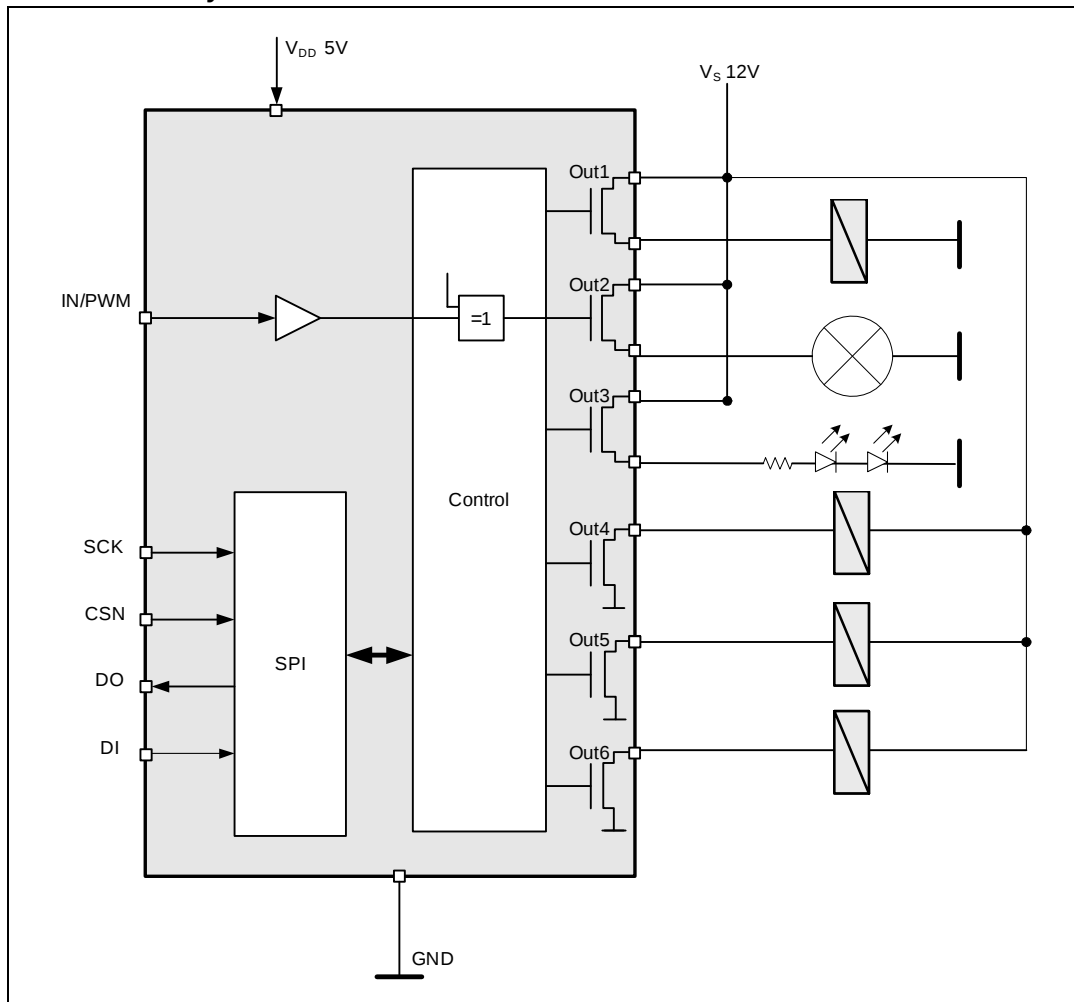
Figure 19. L99MC6 as driver for incandescent bulb, LEDs and high-side or low-side relays
