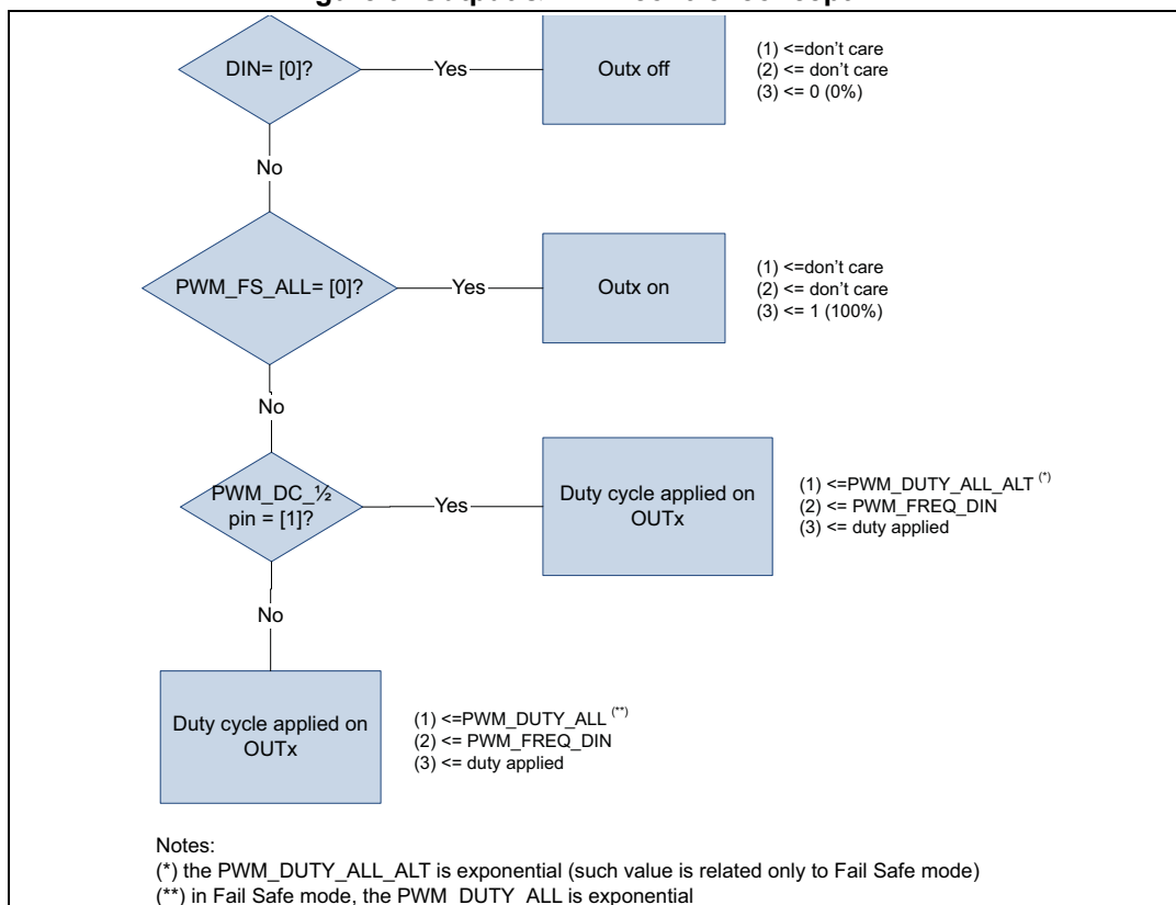
Figure 9. Output &amp; PWM control concept DIN
