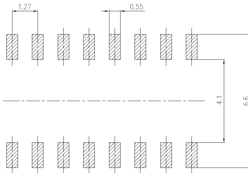
Figure 22. Recommended footprint
