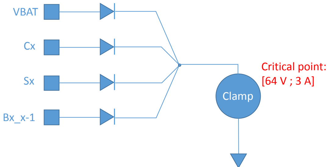
Figure 56. L9963E centralized clamp
