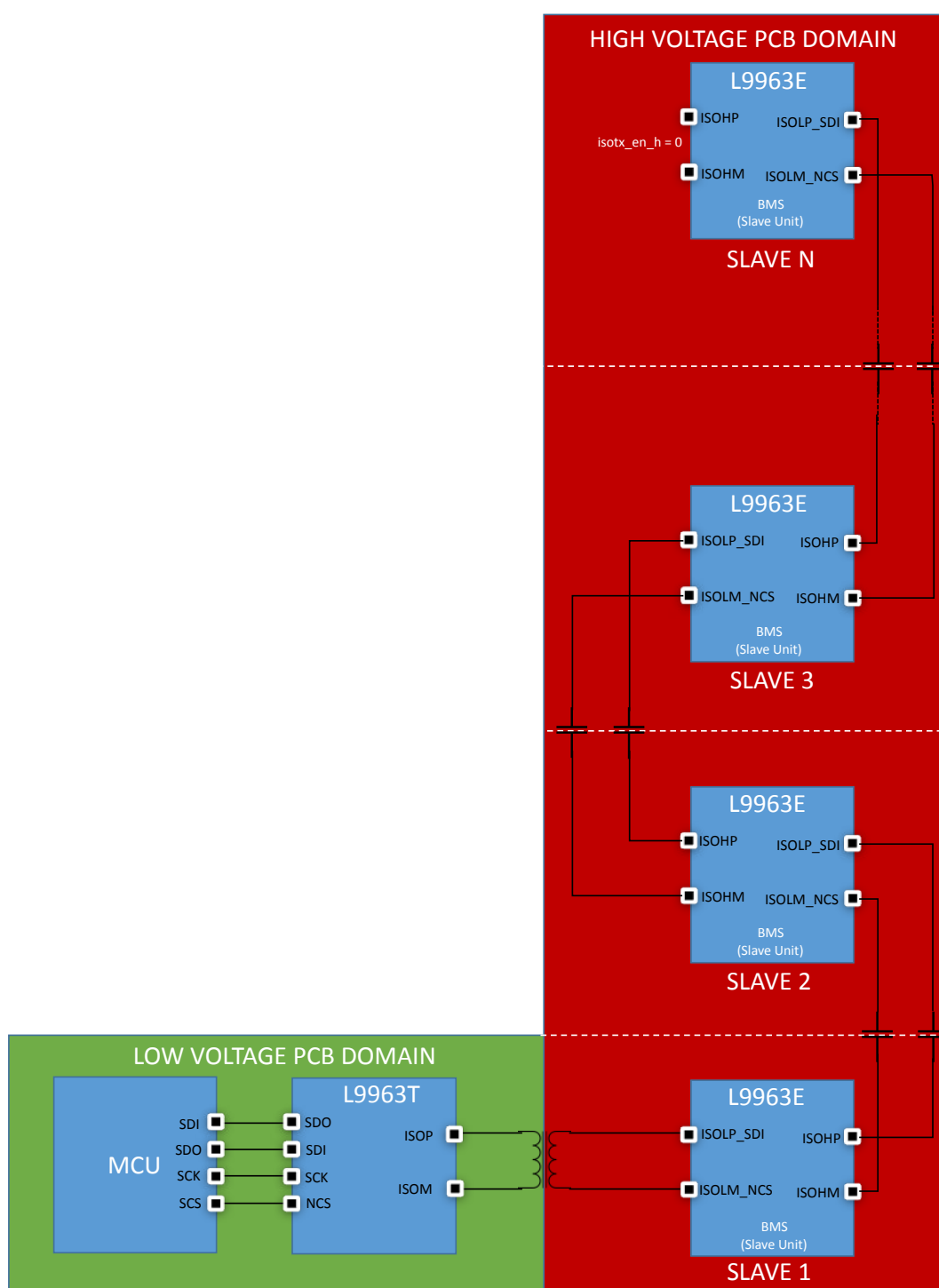
Figure 50. Centralized BMS
