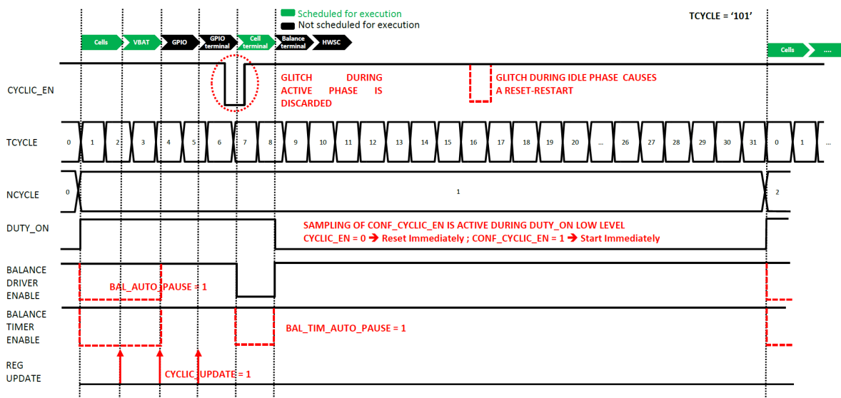
Figure 25. Example of routine execution in normal mode
