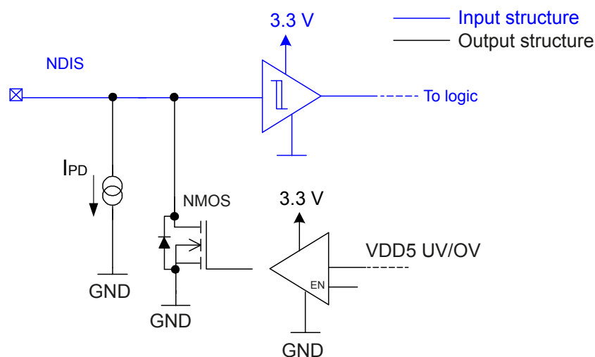
Figure 24. NDIS structure
