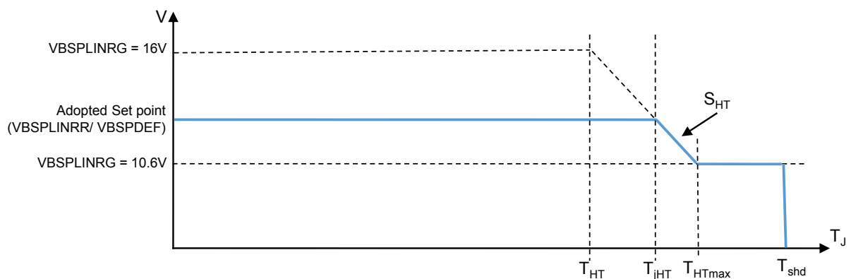
Figure 7. Thermal compensation
