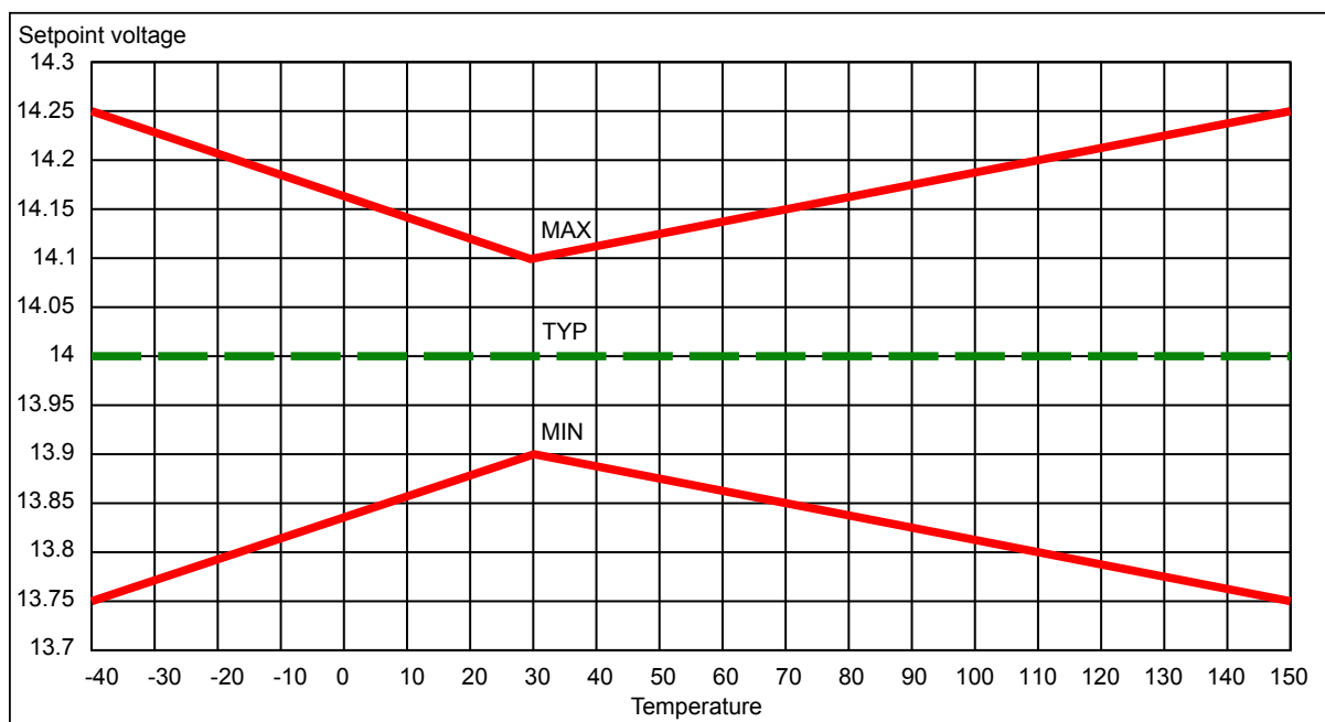
Figure 5. Set point voltage tolerance versus temperature: example with 14V set point (VBSPLINRG or VBSPDEF).
