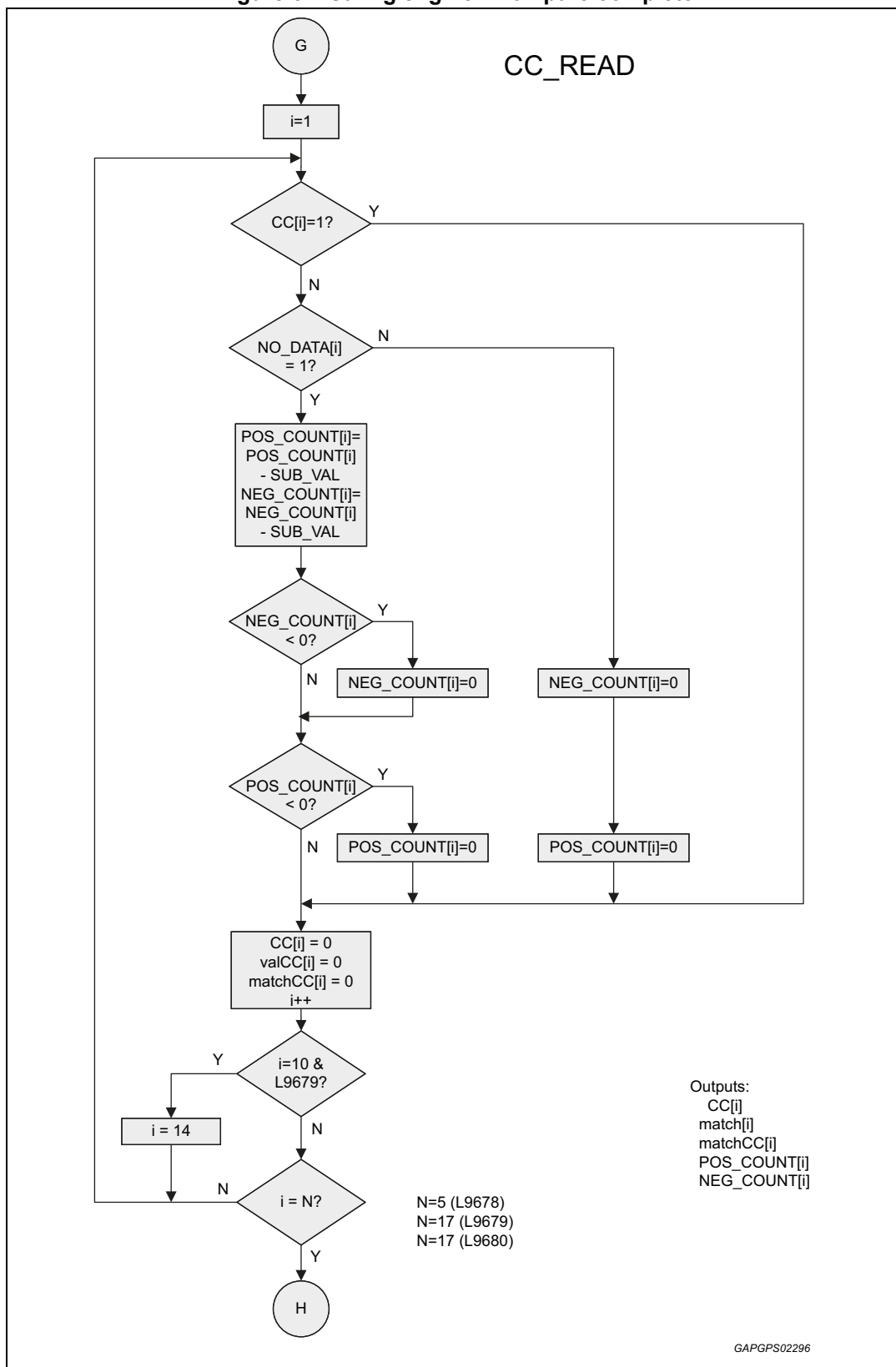
Figure 57. Safing engine - Compare complete
