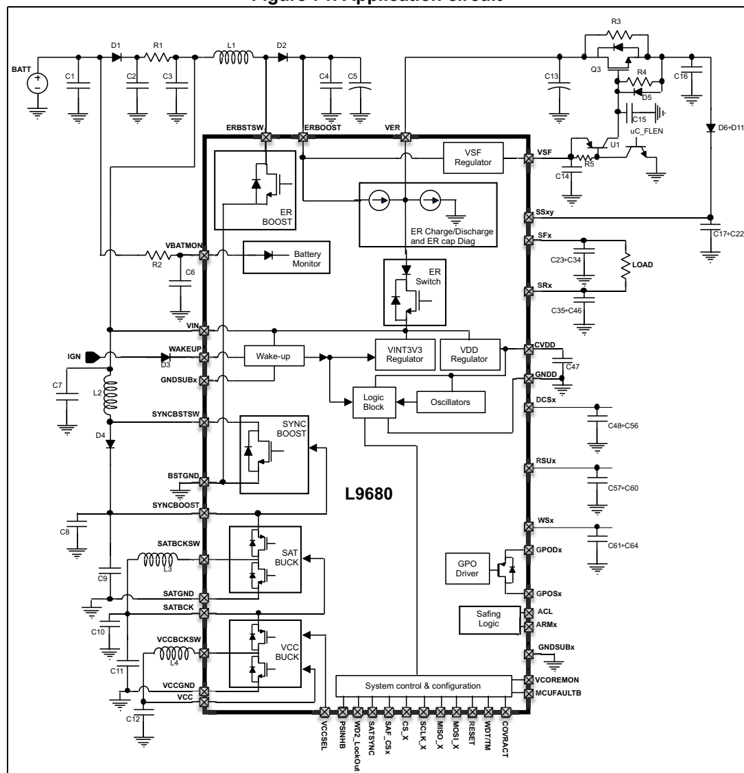
Figure 71. Application circuit
