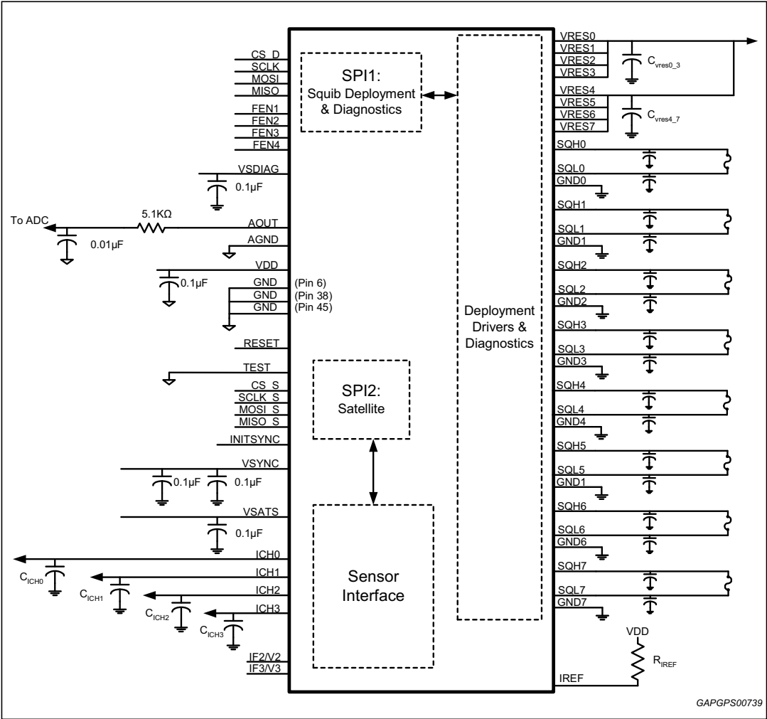
Figure 1. Block diagram
