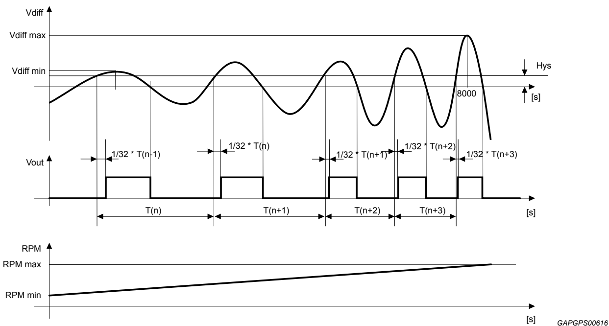
Figure 34. Auto-adaptative time filter behaviour 2
