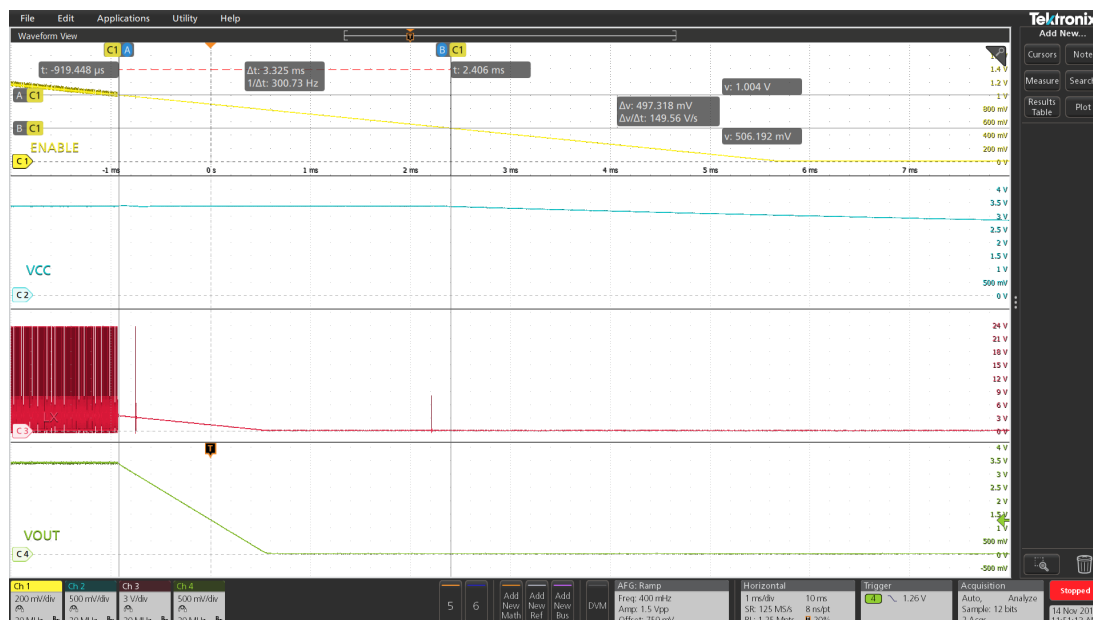
Figure 15. Turn-off example
