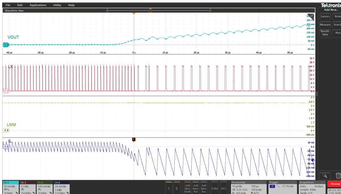
Figure 20. Negative current limit example
