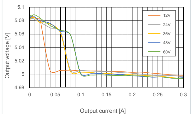
Figure 38. 5 V fix load regulation (LCM)
