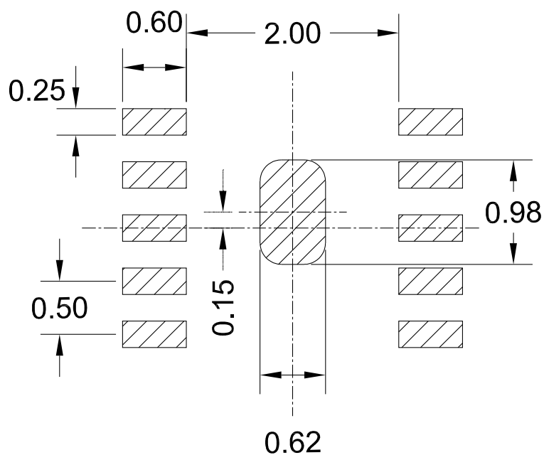
Figure 44. DFN10 (3 x 3 x 0.8 mm) recommended footprint
