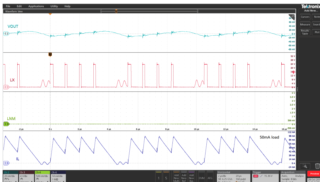
Figure 10. LCM selected, 50 mA load
