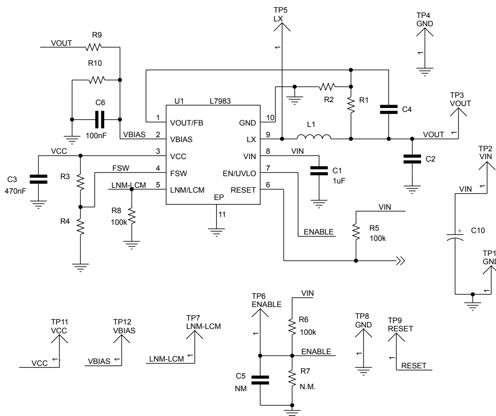
Figure 22. Evaluation board schematic
