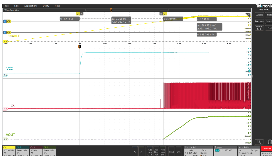
Figure 14. Turn-on example
