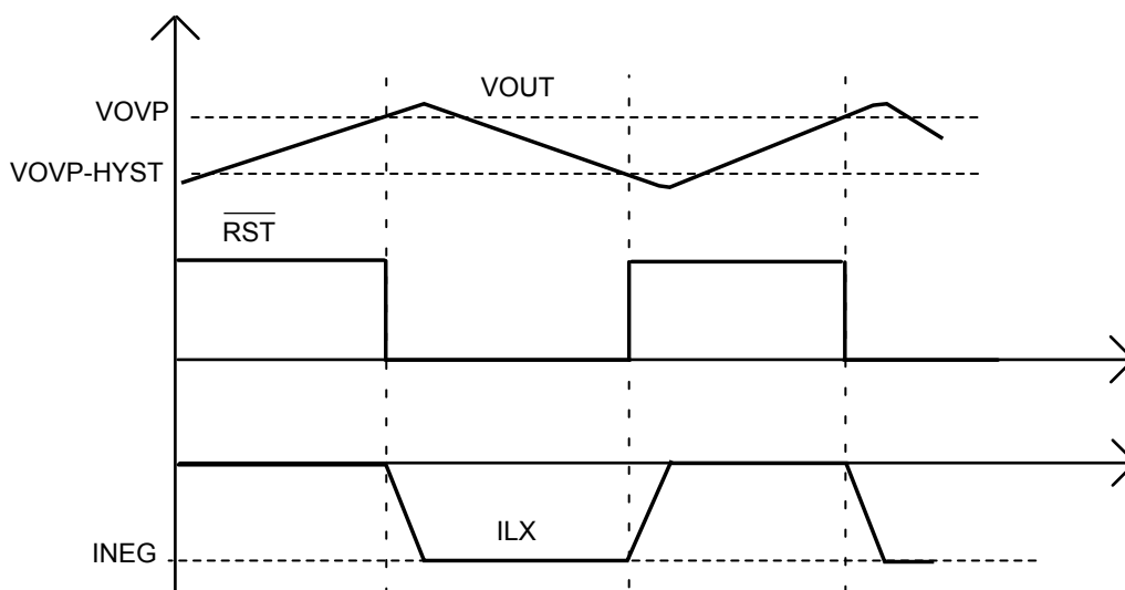
Figure 21. Overvoltage protection
