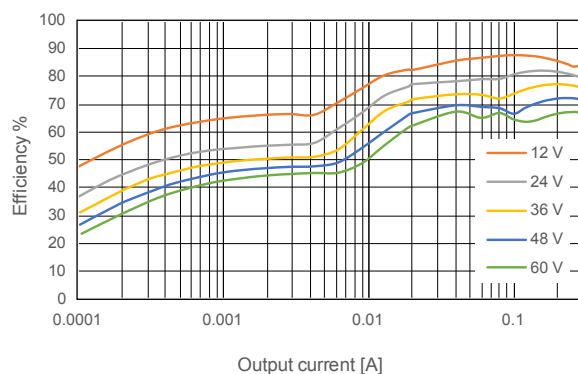
Figure 31. 3.3 V fix efficiency (LCM)
