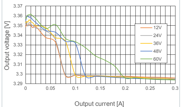
Figure 32. 3.3 V fix load regulation (LCM)
