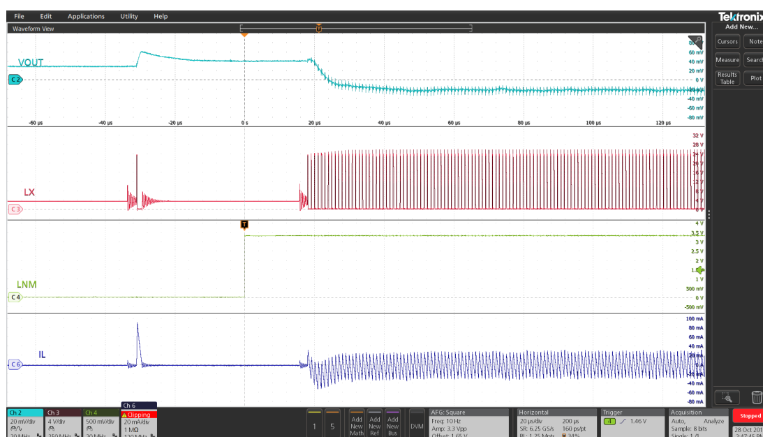
Figure 11. LCM to LNM transition, no load
