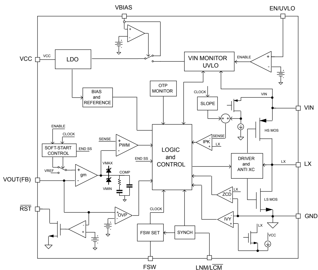
Figure 2. Block diagram
