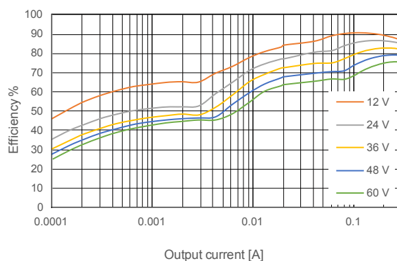
Figure 37. 5 V fix efficiency (LCM)
