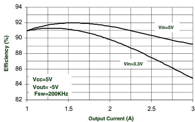
Figure 31. Efficiency vs. Output Current
