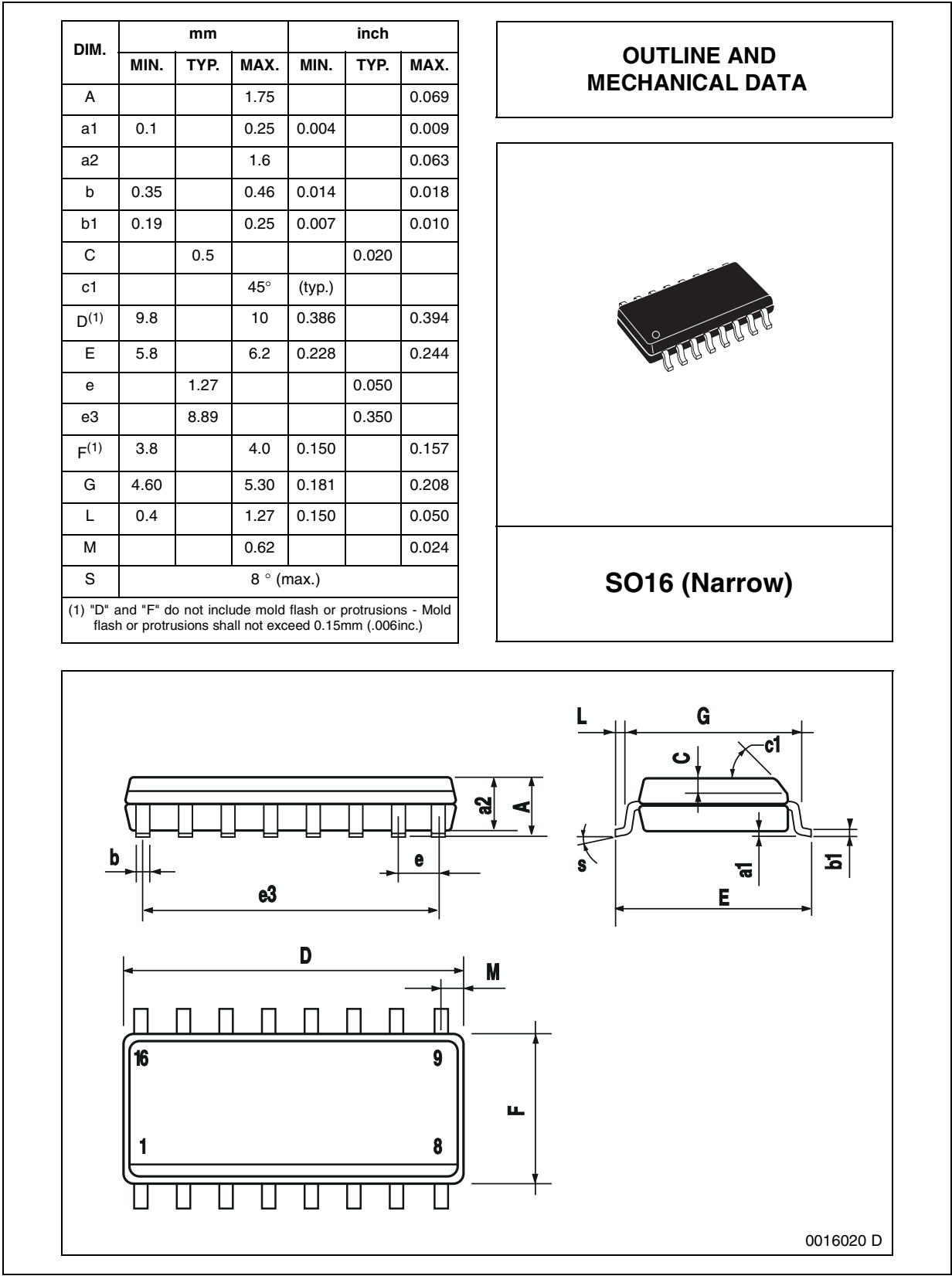
Figure 32. SO-16 (Narrow) Mechanical Data & Package Dimensions
