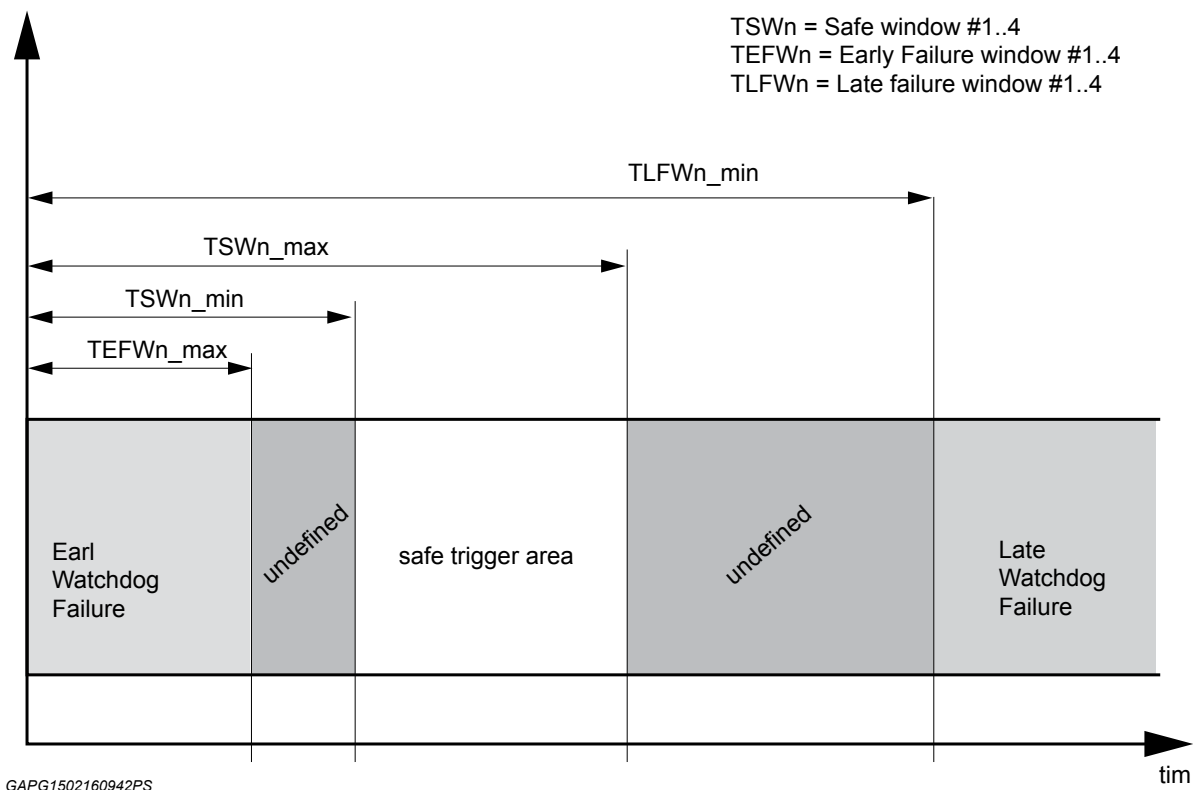
Figure 18. Watchdog Early, Safe and Late window diagram
