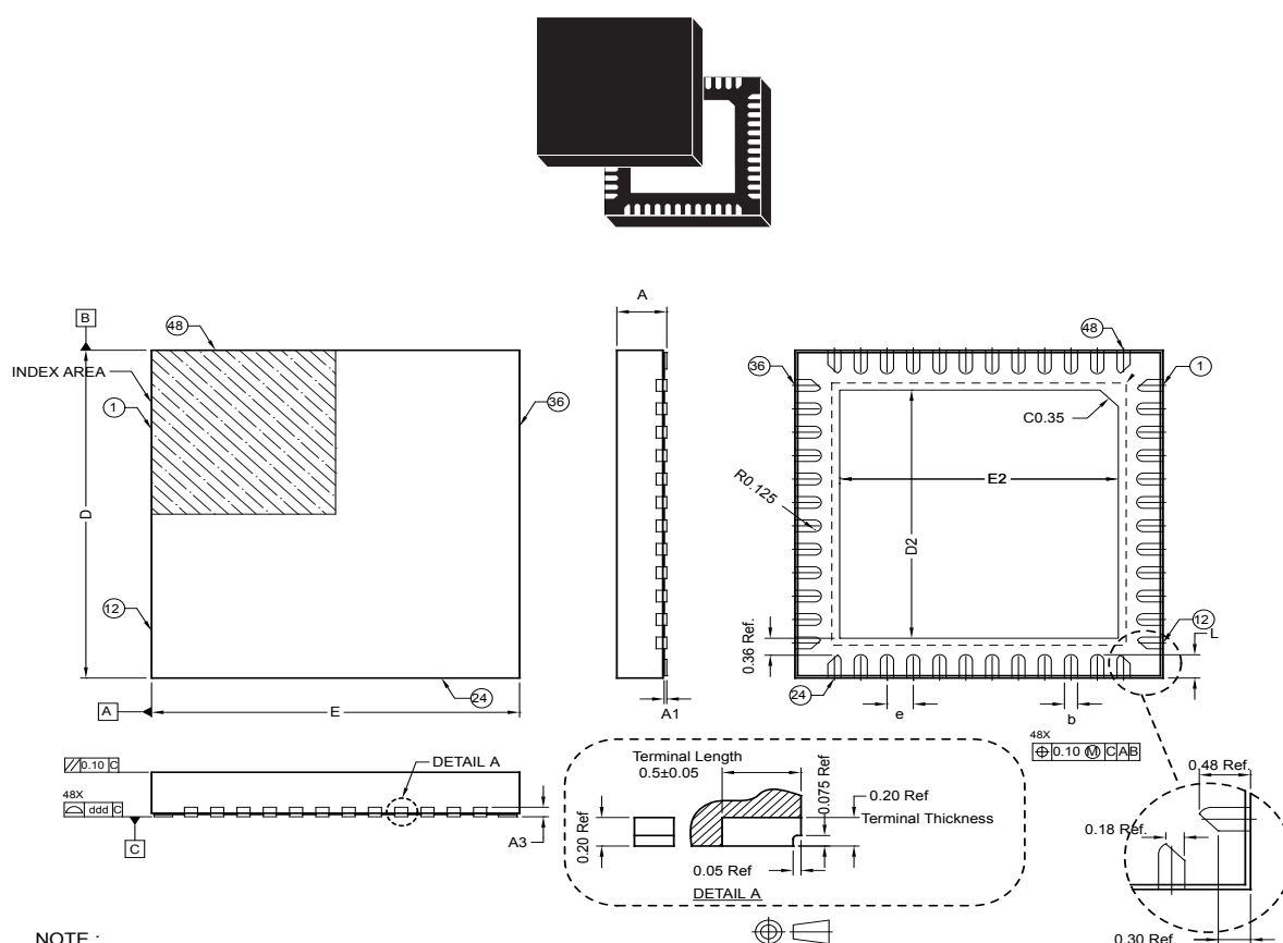
Figure 39. VFQFPN-48 (7x7x1.0 mm - opt. D) package outline
