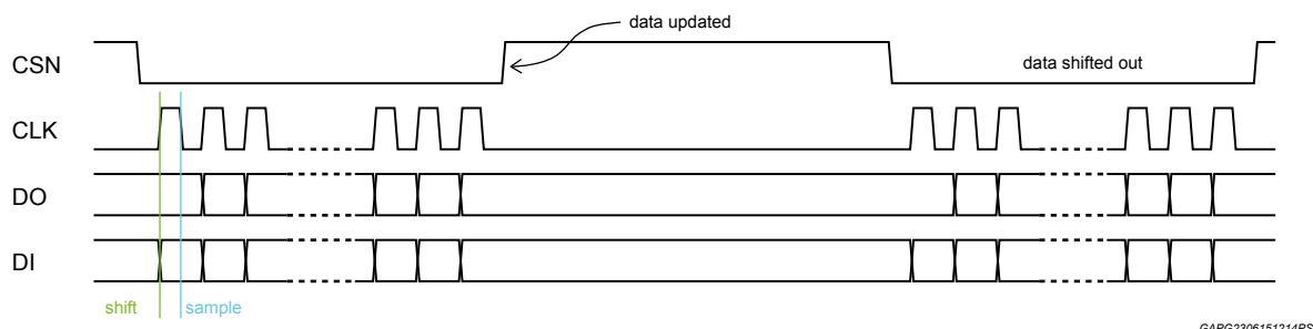
Figure 23. SPI diagram
