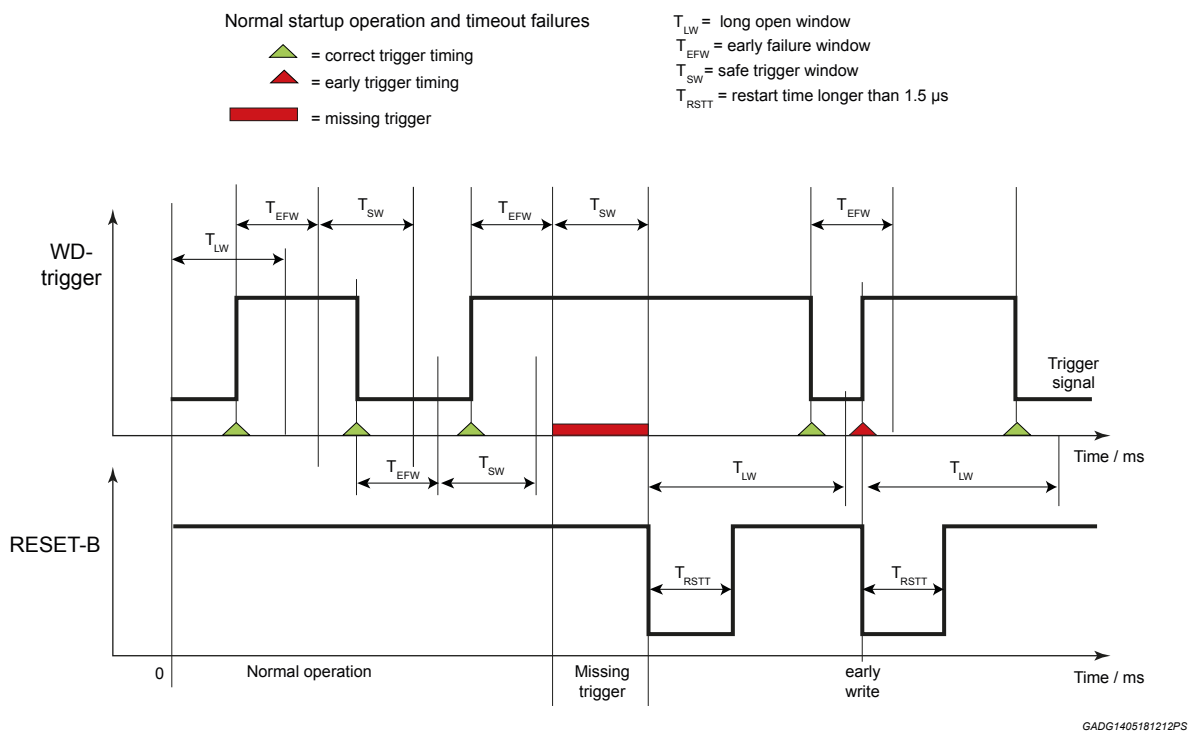
Figure 18. Watchdog Early, Safe and Late window diagram
