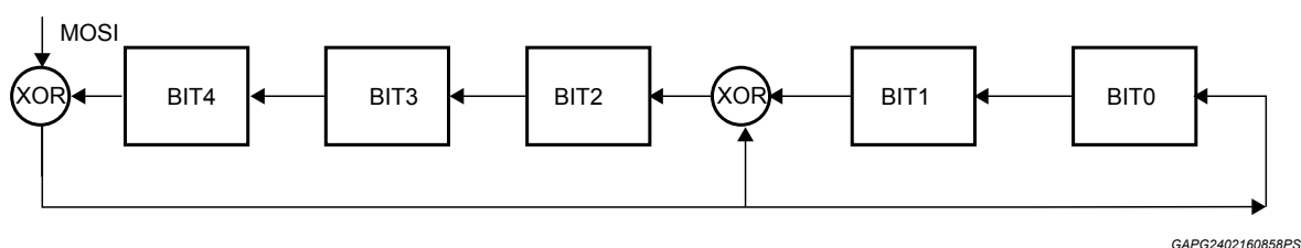
Figure 25. Structure of CRC generator
