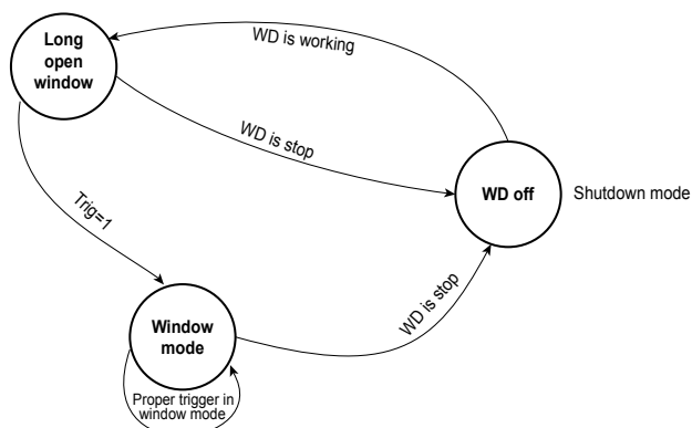
Figure 15. Watchdog behavior
