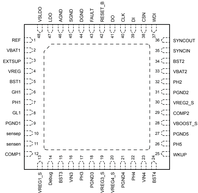
Figure 3. Pin out (top view)
