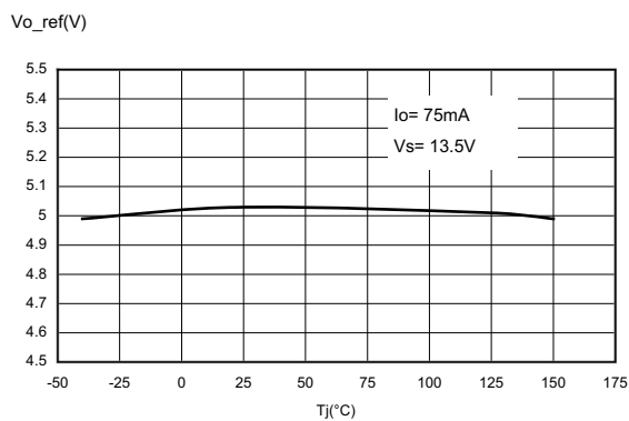
Figure 3. Output voltage vs. T j
