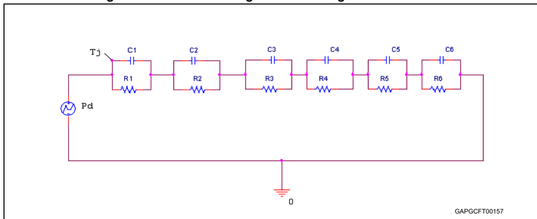
Figure 32. Thermal fitting model of Vreg in PowerSSO-12
