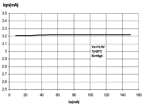
Figure 7. Current consumption vs. output current
