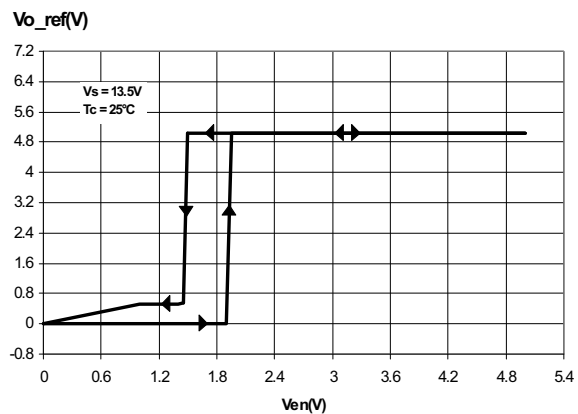
Figure 5. Output voltage vs. V_{En}
