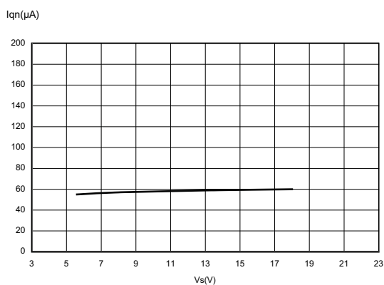
Figure 9. Current consumption vs. input voltage ( I_o = 0.1 mA)
