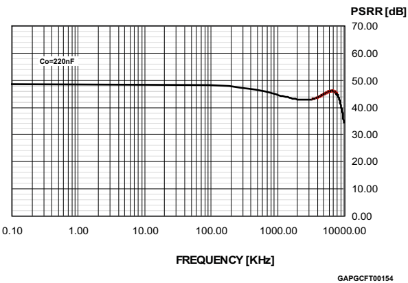
Figure 23. PSRR
