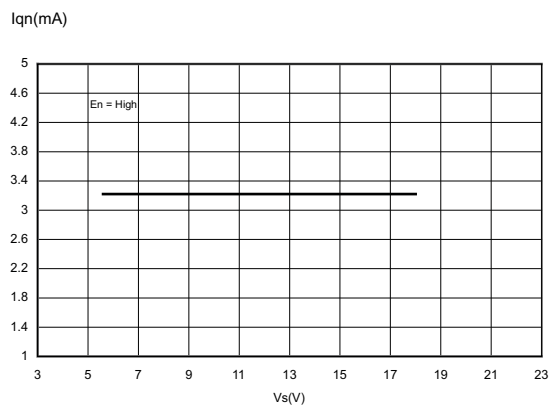
Figure 10. Current consumption vs. input voltage ( I_o = 75 mA)
