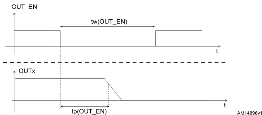
Figure 8. Output channel enable timing
