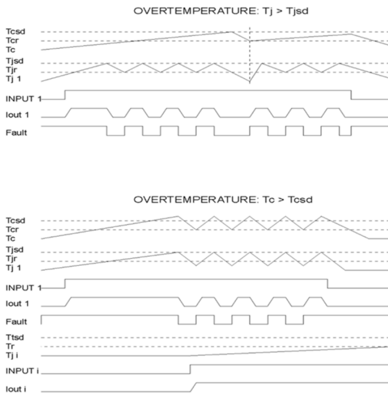
Figure 18. Thermal protection
