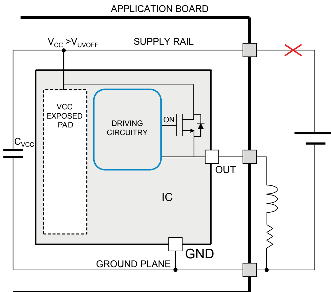
Figure 8. VCC disconnection
