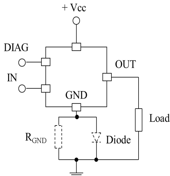
Figure 3. Reverse polarity
