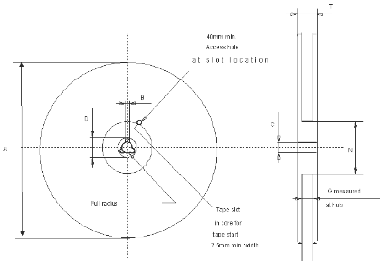
Figure 16. PowerSSO-24 reel shipment
