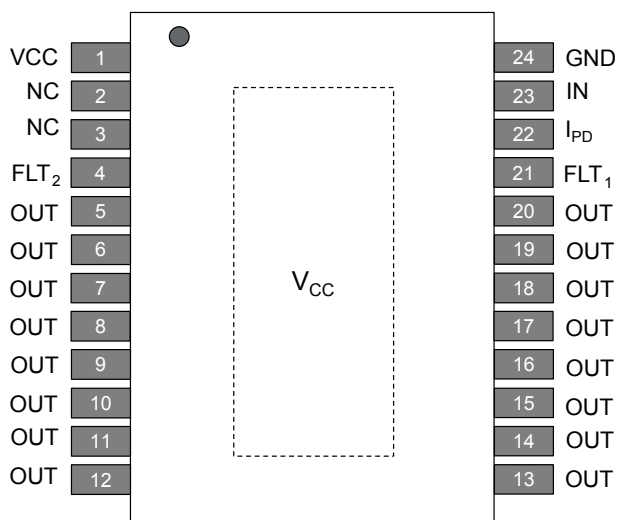
Figure 2. Pin connections (top through view)
