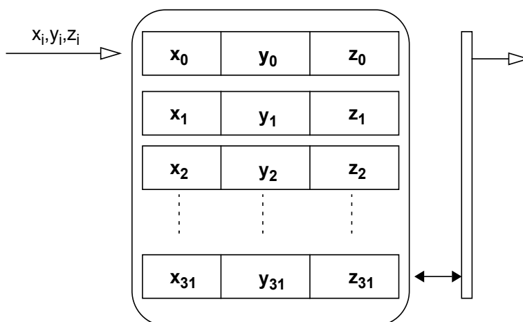
Figure 10. FIFO mode
