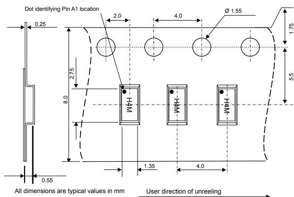
Figure 12. μQFN-10L tape and reel specification
