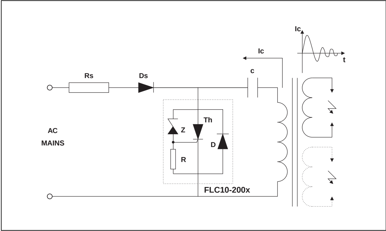
Figure 5. Basic application
