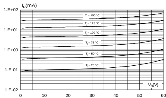
Figure 3: Reverse leakage current versus reverse voltage applied (typical values, per diode)
