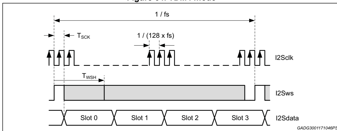
Figure 64. TDM4 mode
