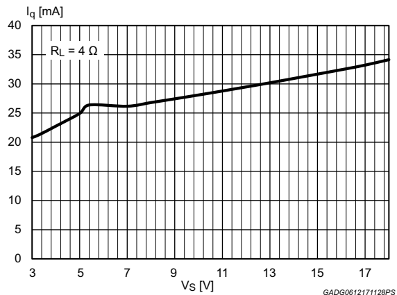
Figure 35. Quiescent current vs. supply voltage
