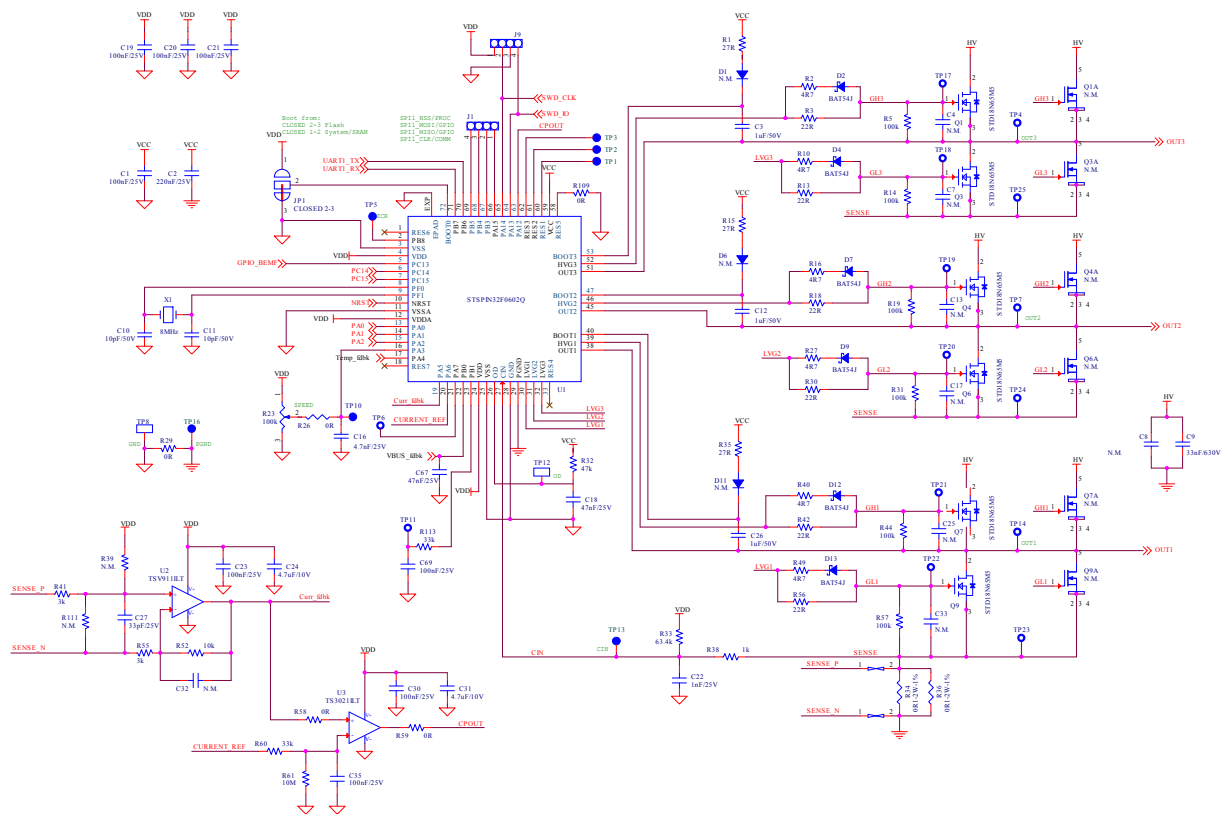
Figure 1. EVSPIN32F06Q2S1 schematic – Driver output stages
