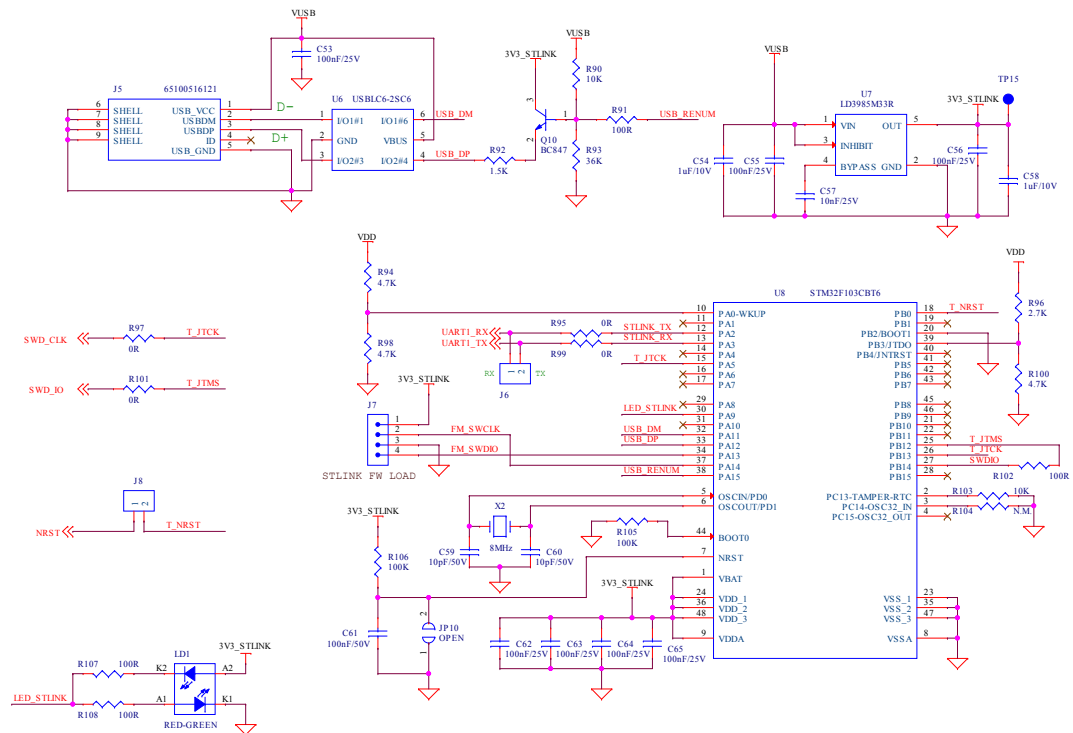
Figure 4. EVSPIN32F06Q1S3 schematic – STLINK debugger
